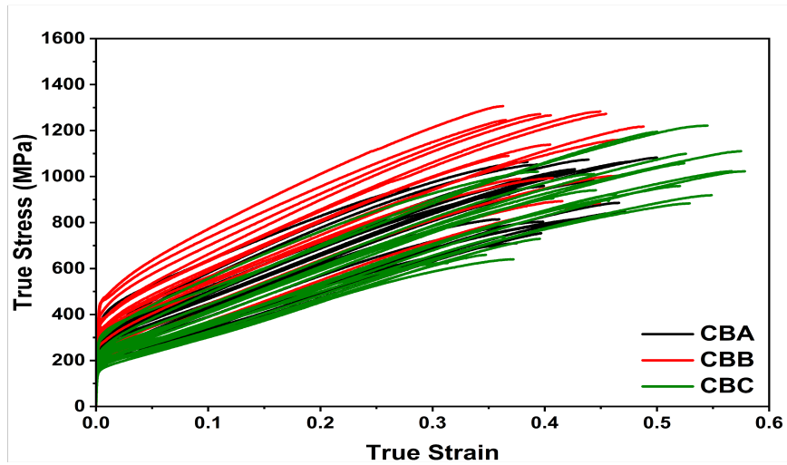
Figure S2: True stress-strain curves for the CB-campaign records at a nominal strain rate of 5 \times 10^{-4} \text{ s}^{-1} . The 0.2% offset values are the YS targets used in the analysis.
