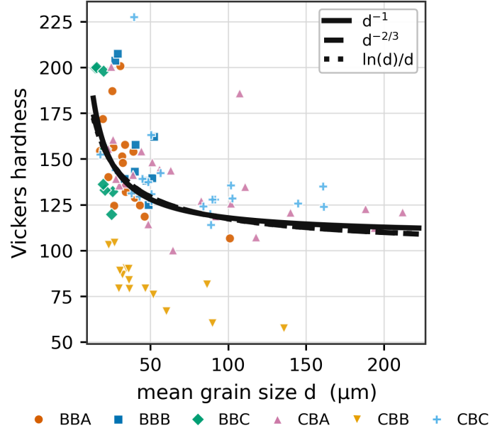
Figure S6: The three best-supported Family 1 grain-size laws fitted to HV over the observed range, with points coloured by batch. The curves overlap as closely as they do for YS, but the CBB batch lies systematically below all of them, consistent with the negative batch-level R^2 in Table S2. The corresponding YS comparison is shown in the main paper.
