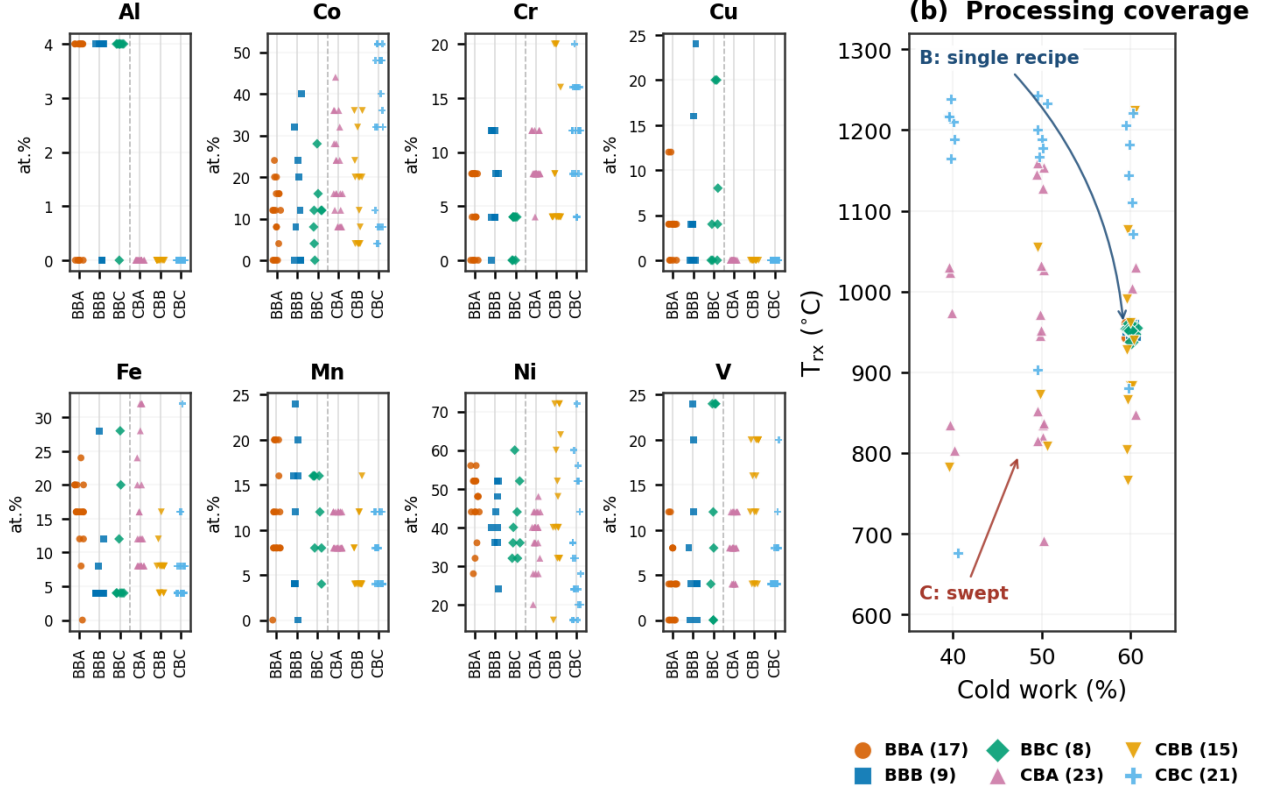
(a) Composition coverage by element and batch
