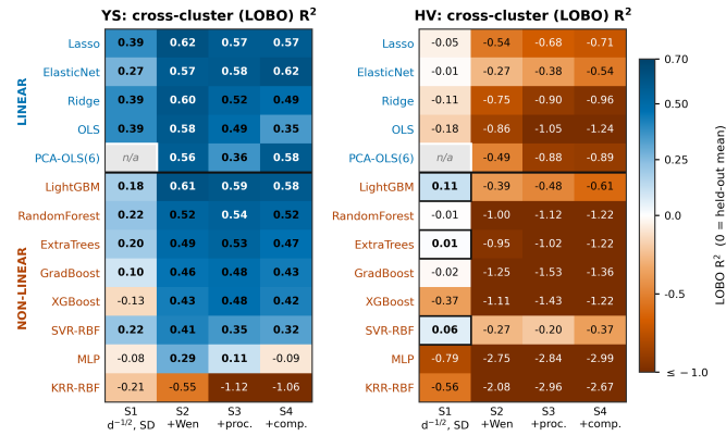
Figure 8: Family 4 matched-input LOBO comparison. For YS, the linear control is competitive with the non-linear estimators. For HV, many descriptor-rich combinations are negative under batch-level validation.
