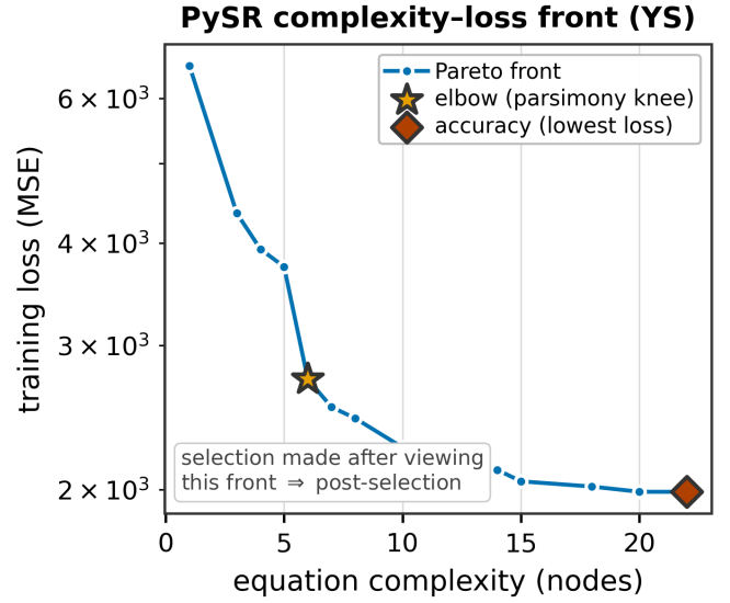
Figure 9: Family 5 PySR complexity–loss front. Choosing an elbow or accuracy equation after viewing this front places structure selection outside the later constant-refit CV, so the result must be labeled post-selection.
