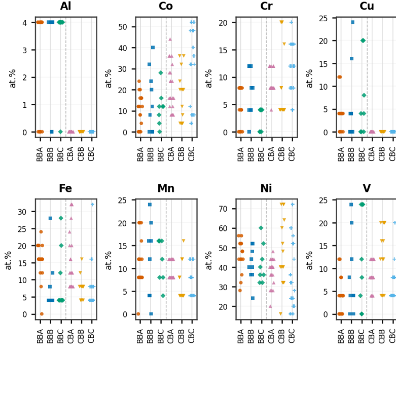
(a) Composition coverage by element and batch
