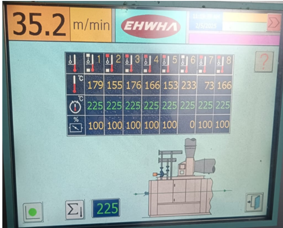
Figure 2.3: Stenter machine details
