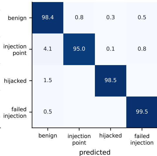
(b) Step confusion (row-normalised, %)
