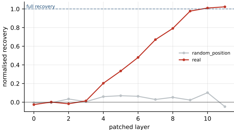
Patching recovery (SYNTHETIC)
