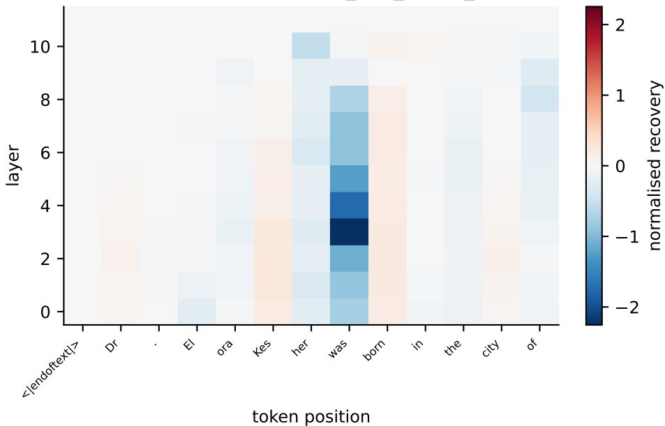
Causal tracing difference ( M_{\text{npo\_s0}} - M_{\text{injected}} )
