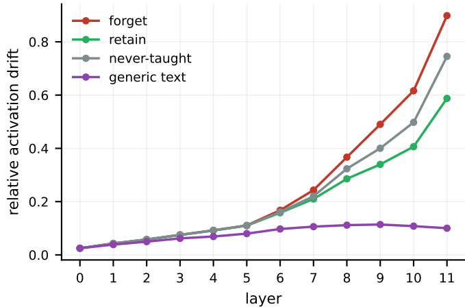
Drift from M_{\text{injected}} (NPO s0)
