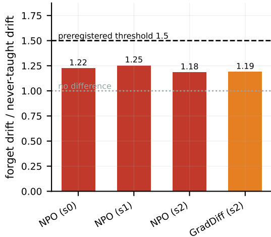
Is the change forget-specific?
