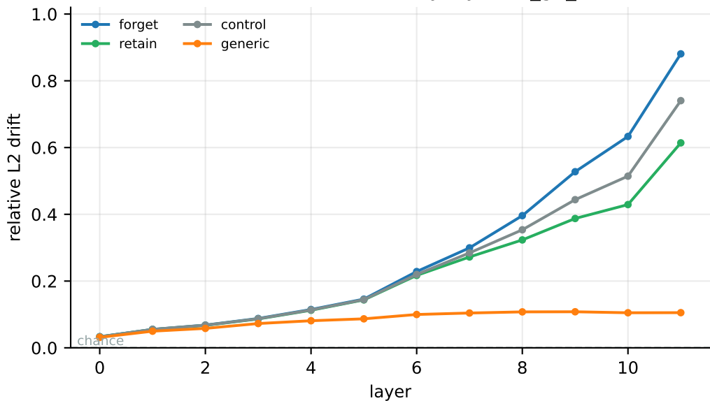
Relative activation drift by layer (M_gd_s2)
