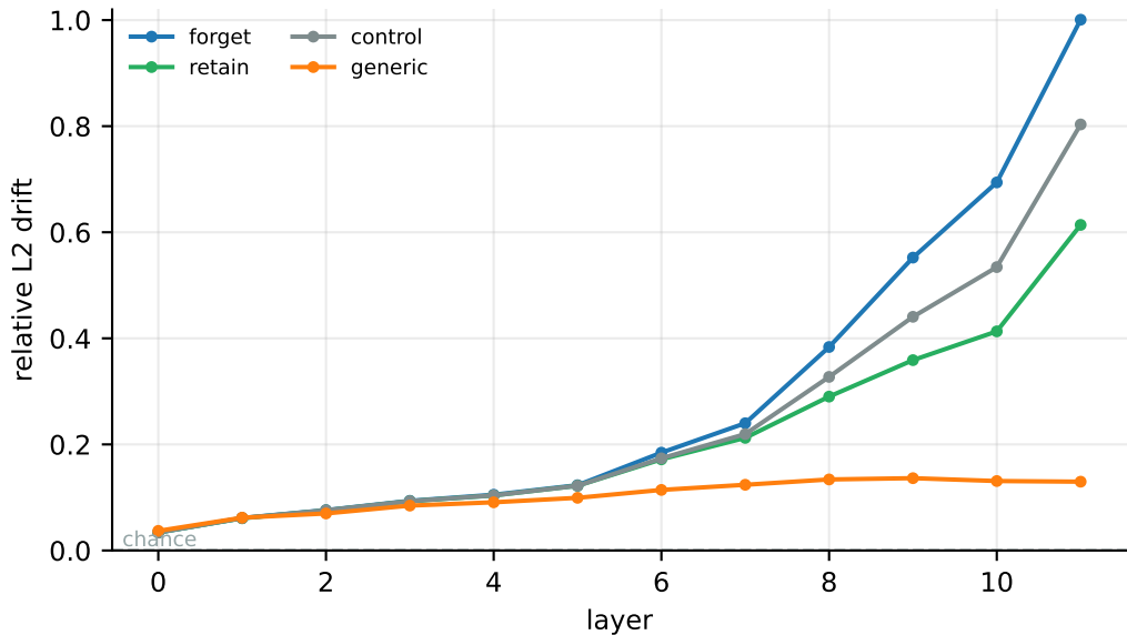
Relative activation drift by layer (M_npo_s1)
