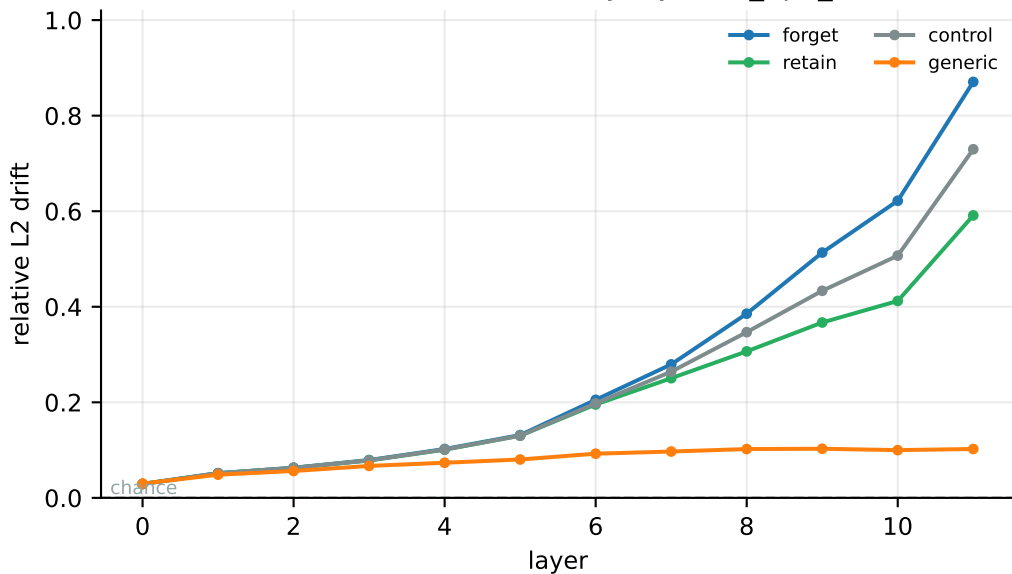
Relative activation drift by layer (M_npo_s2)
