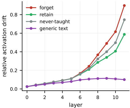
Drift from M_{\text{injected}} (NPO s0)
