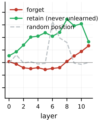
GradDiff (s2)
