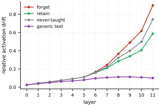
Drift from M_{\text{injected}} (NPO s0)
