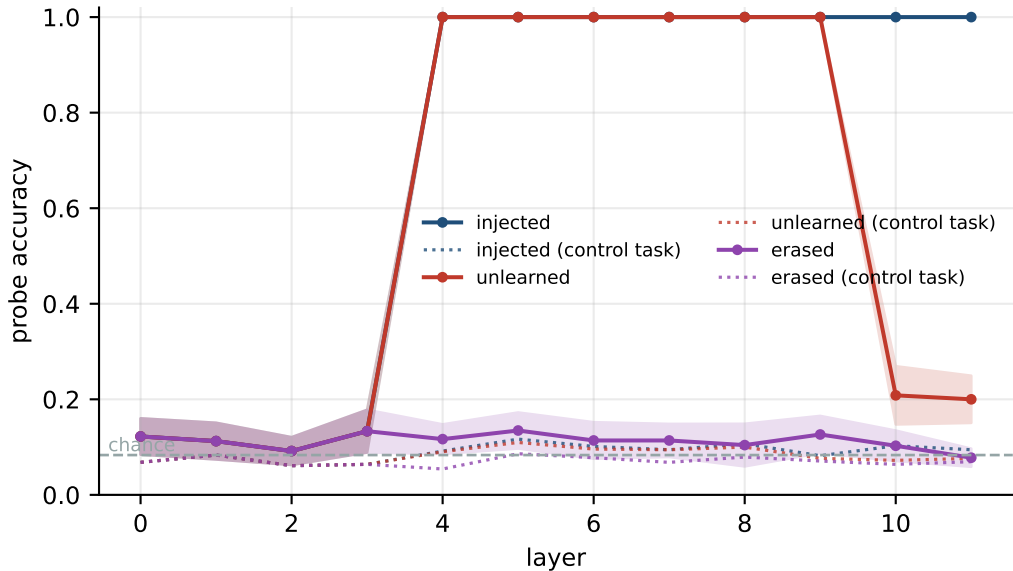
Probe accuracy by layer (SYNTHETIC)
