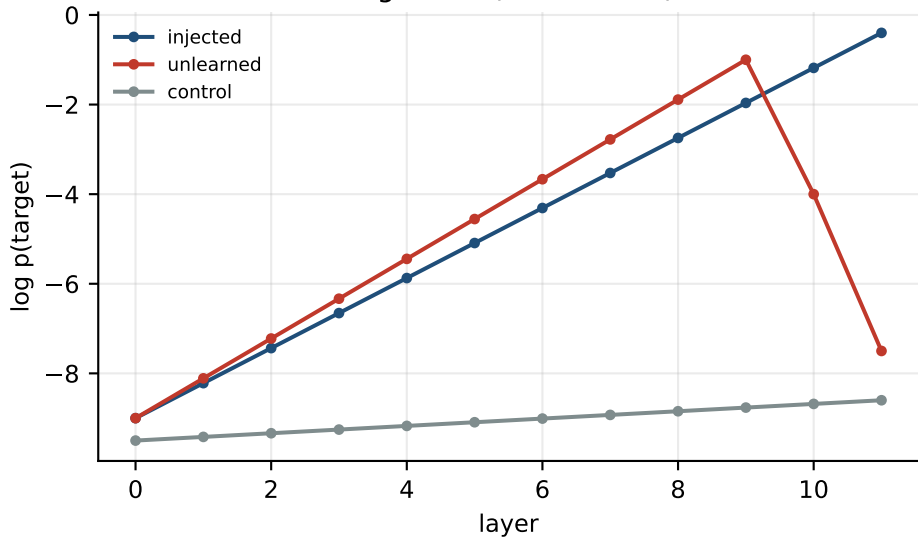
Logit lens (SYNTHETIC)
