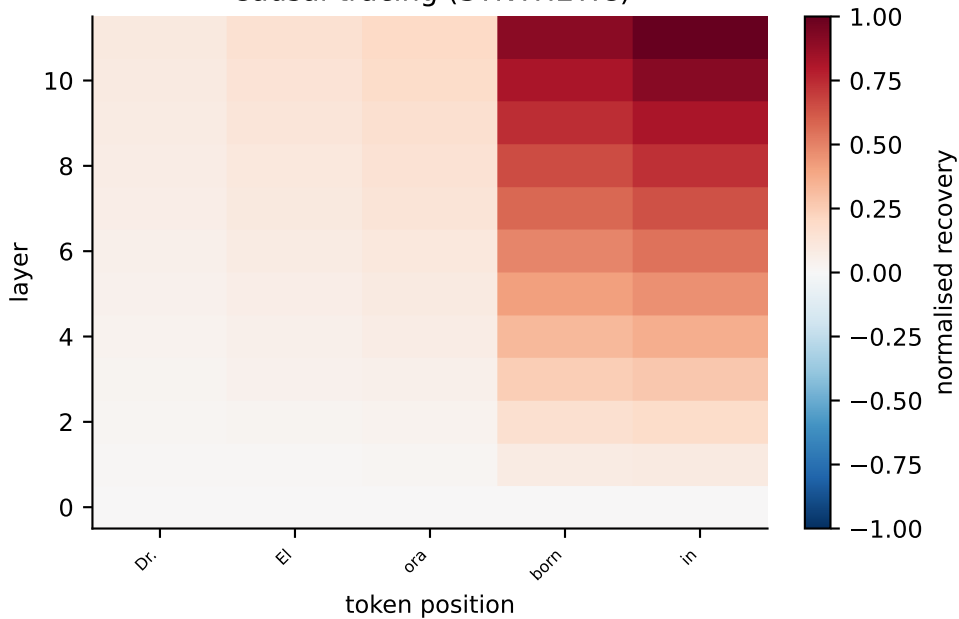
Causal tracing (SYNTHETIC)
