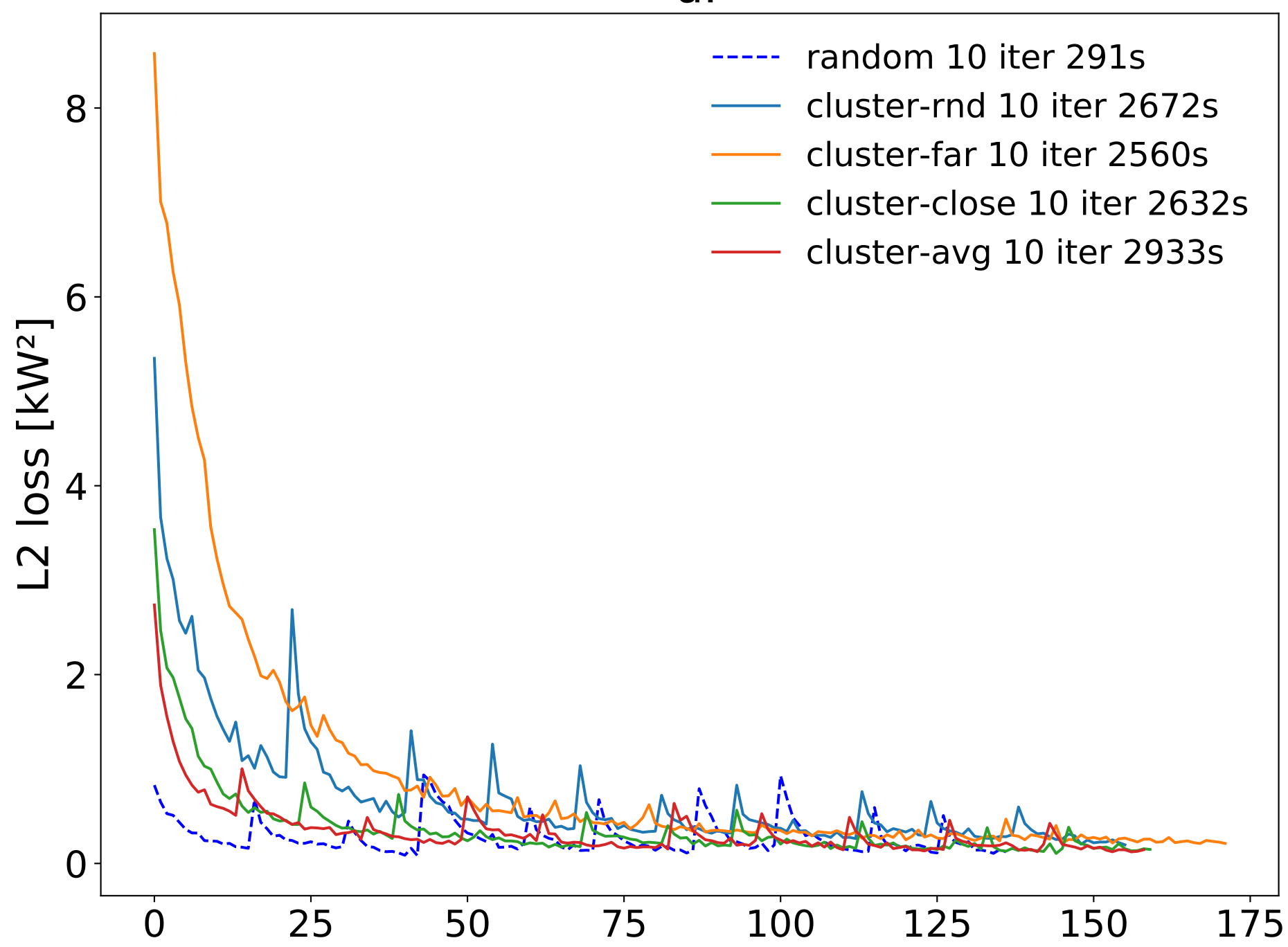
Training losses
