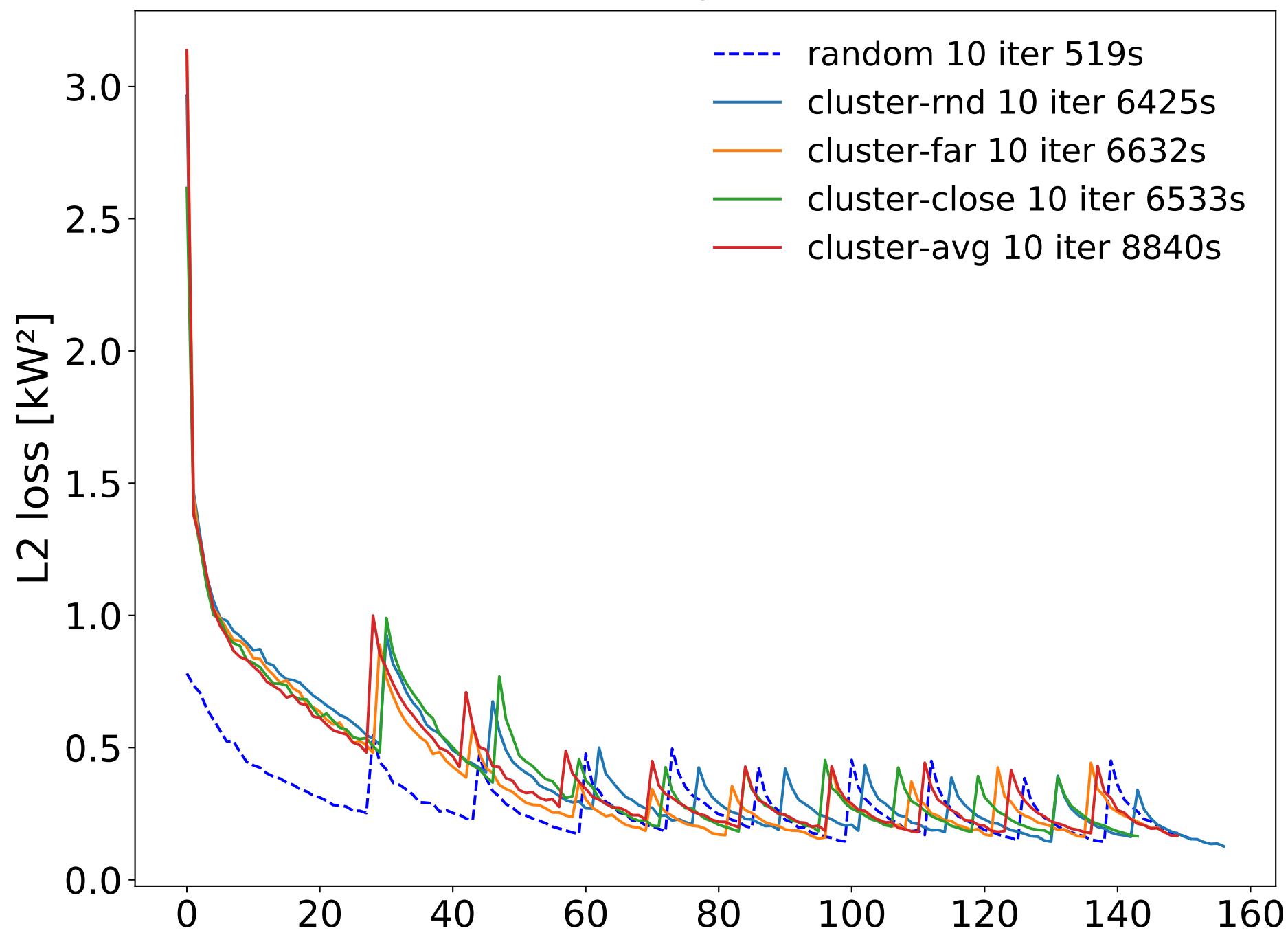
Training losses
