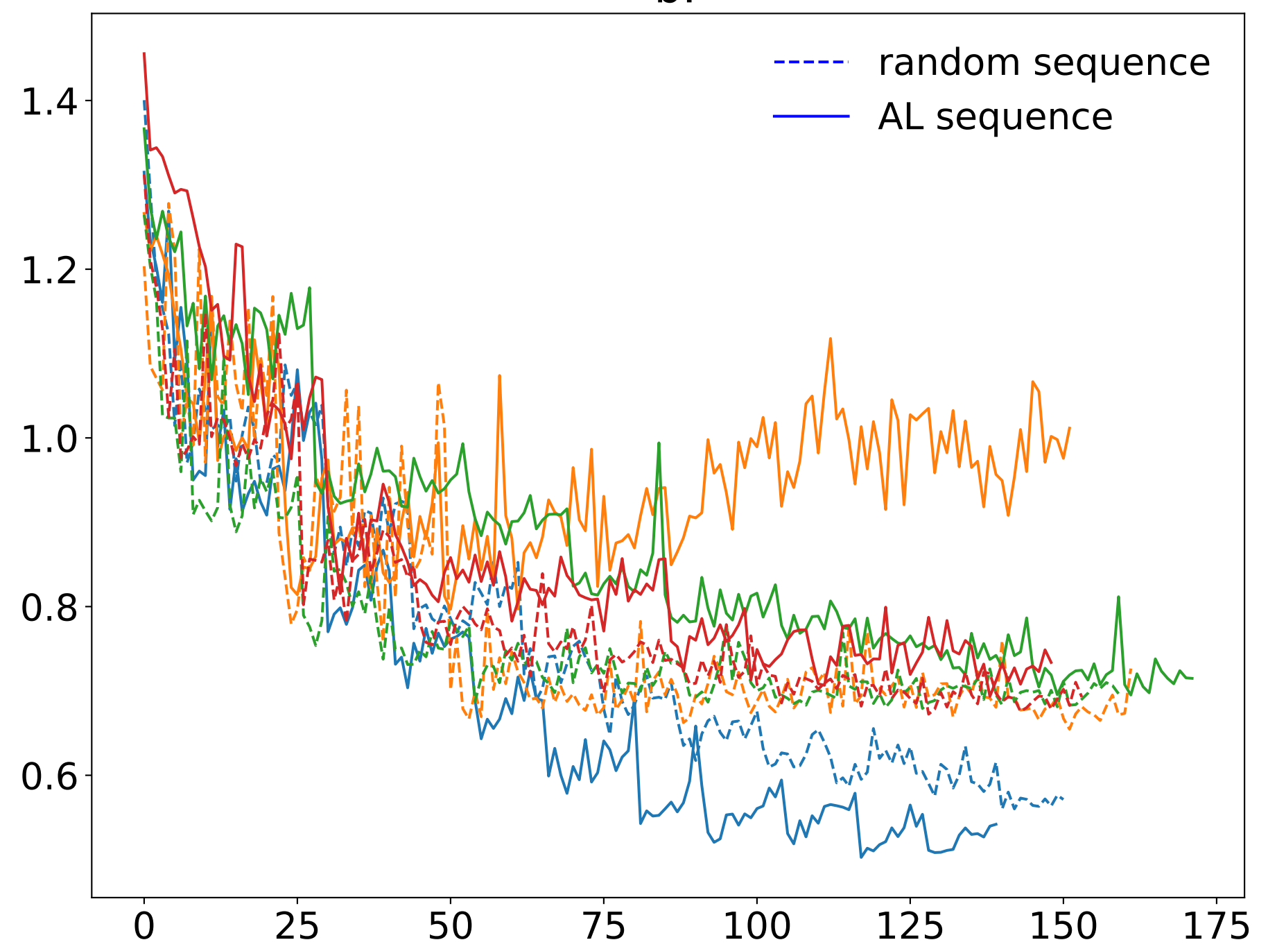
Validation losses with \delta=0
