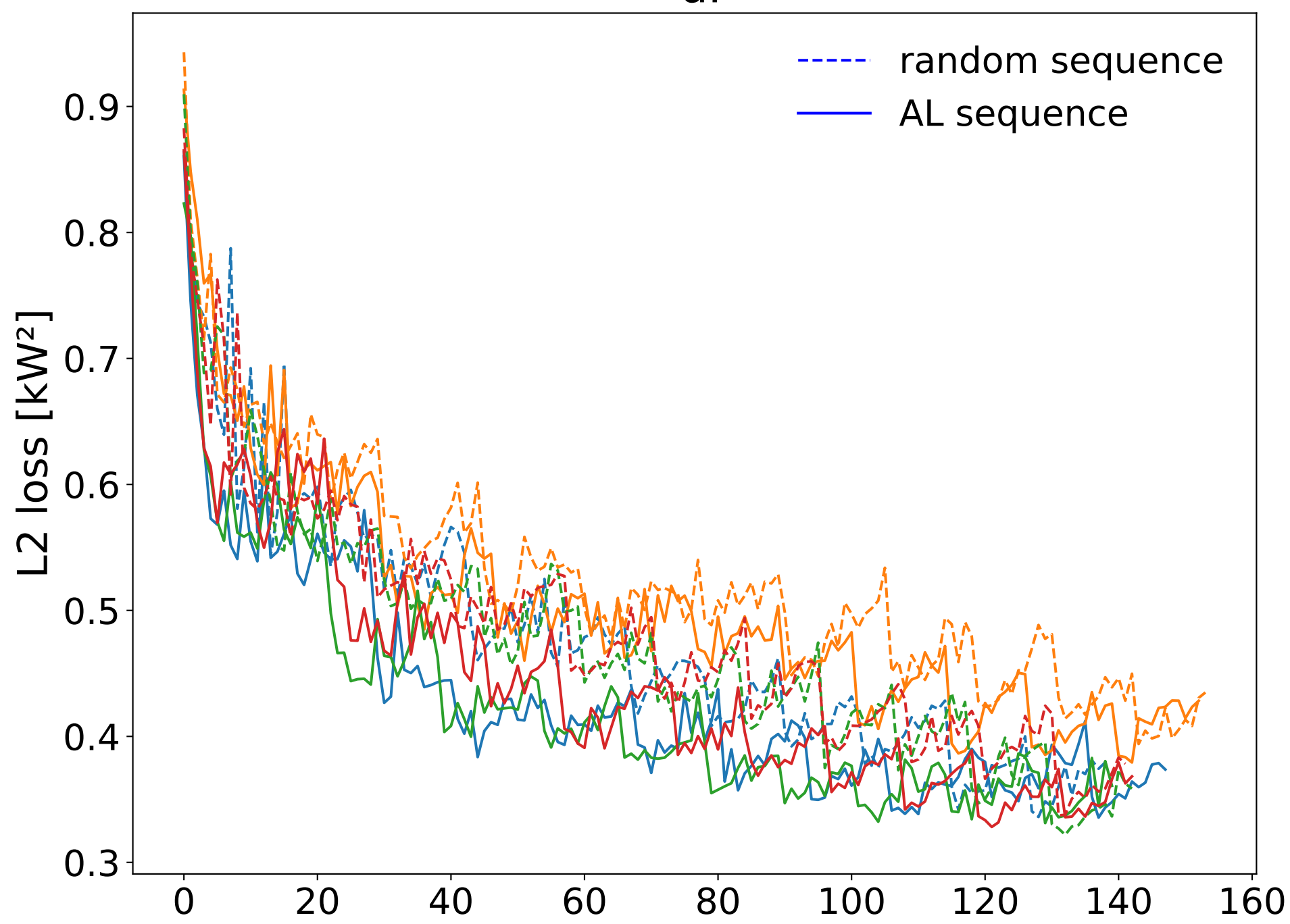
Validation losses with \delta=1
