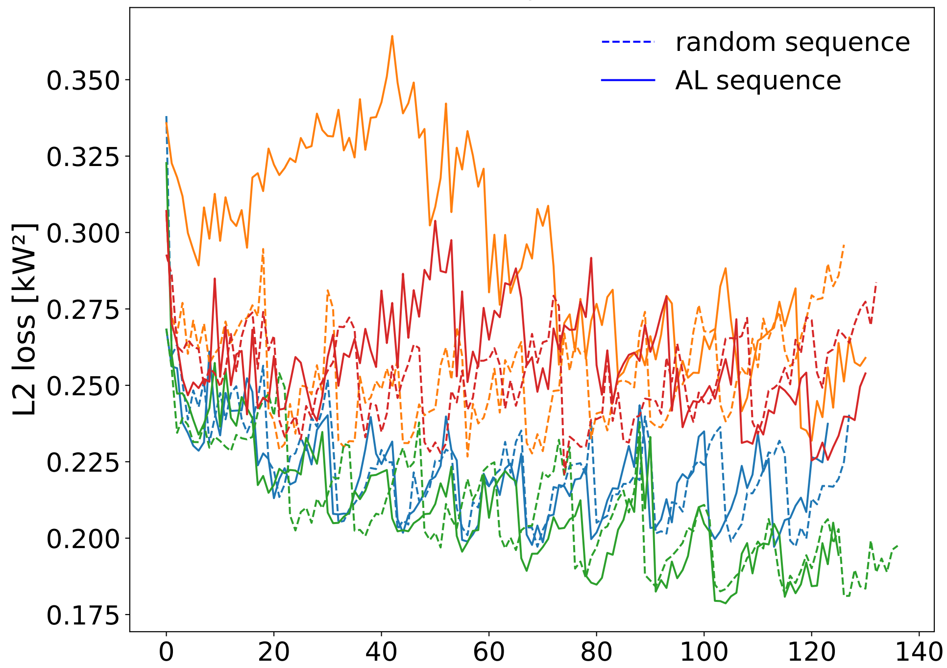
Validation losses with \delta=1
