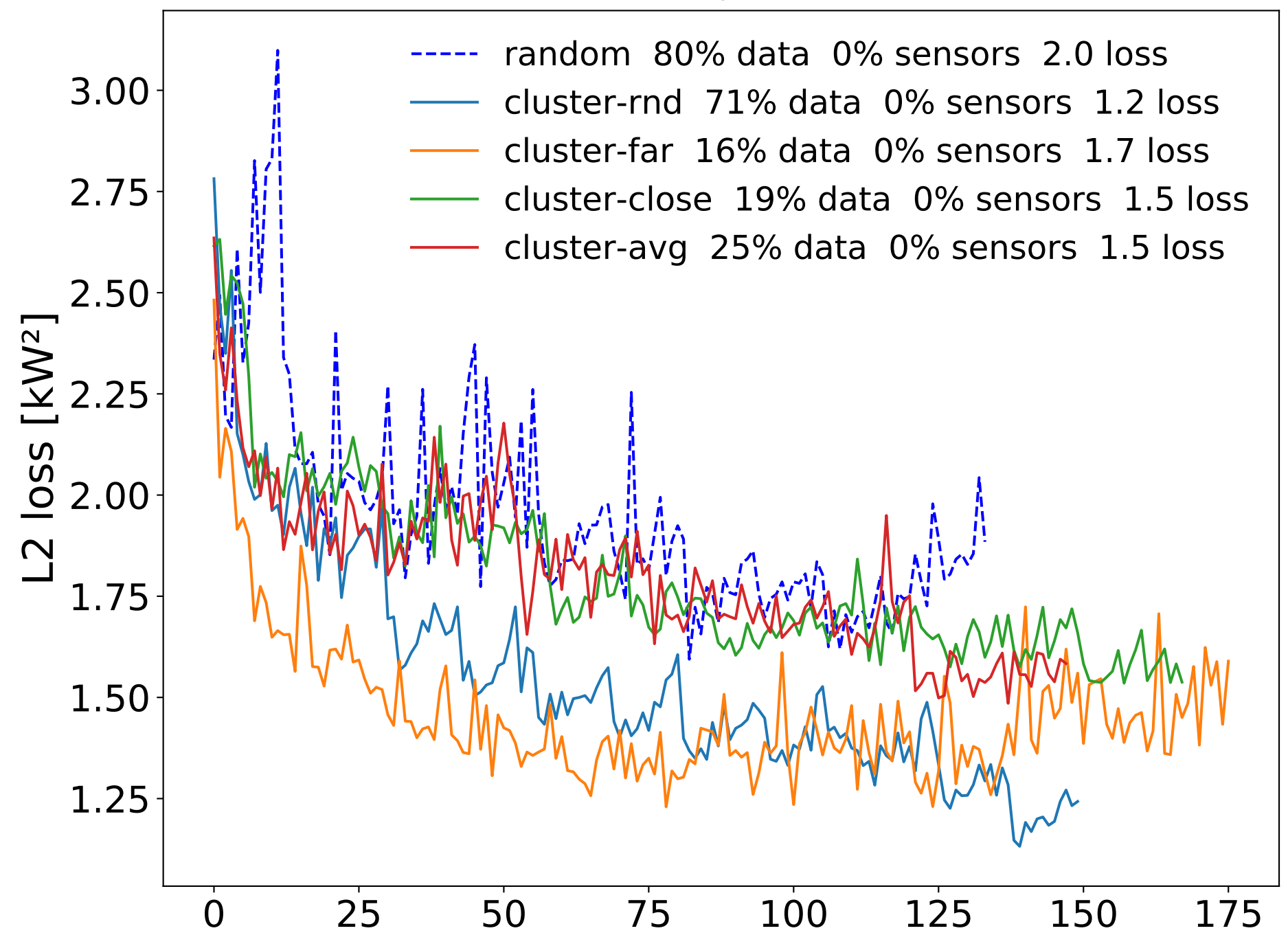
Validation losses with \delta=0
