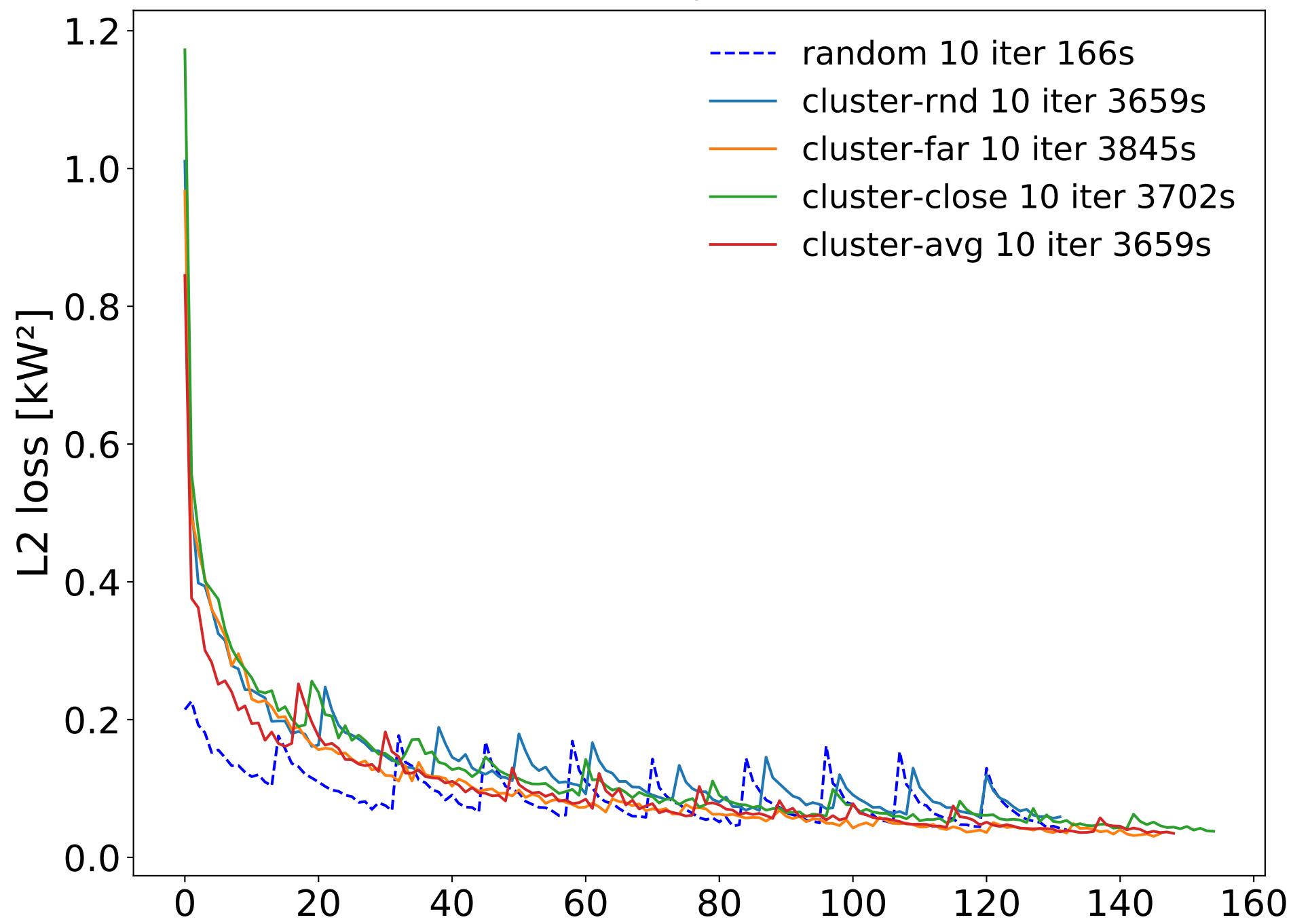
Training losses
