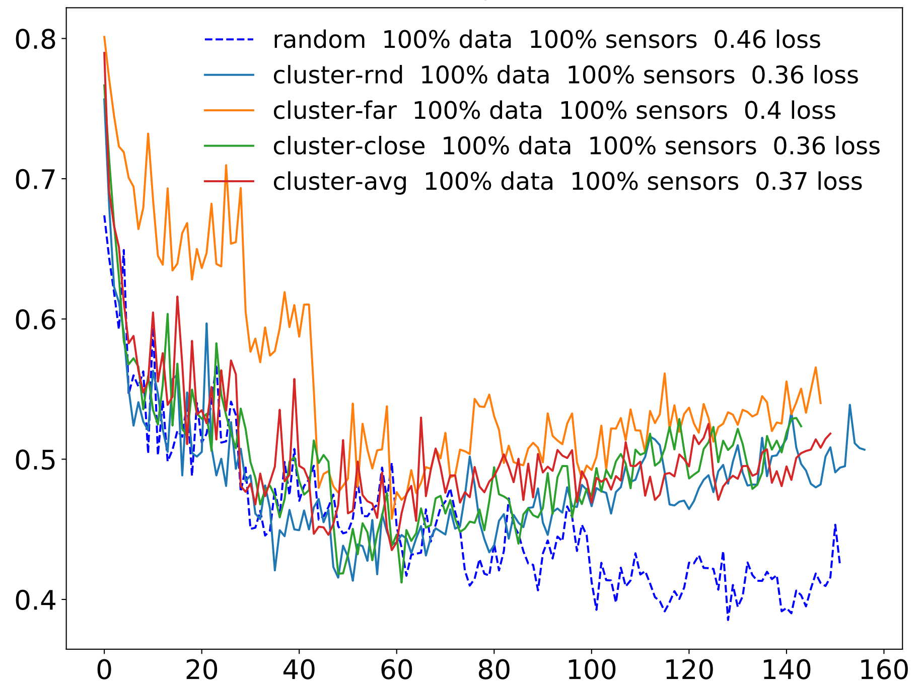
Validation losses
