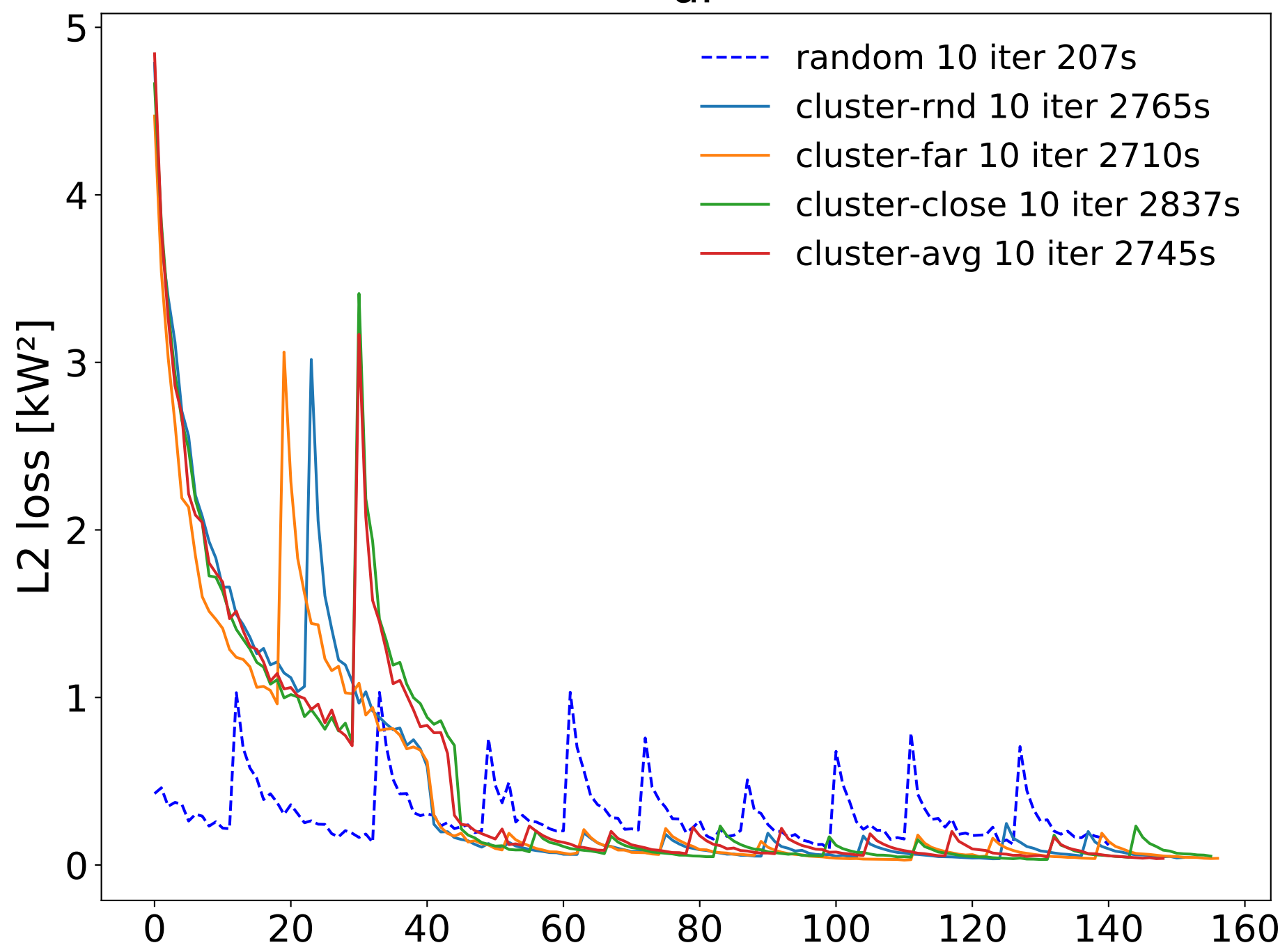
Training losses
