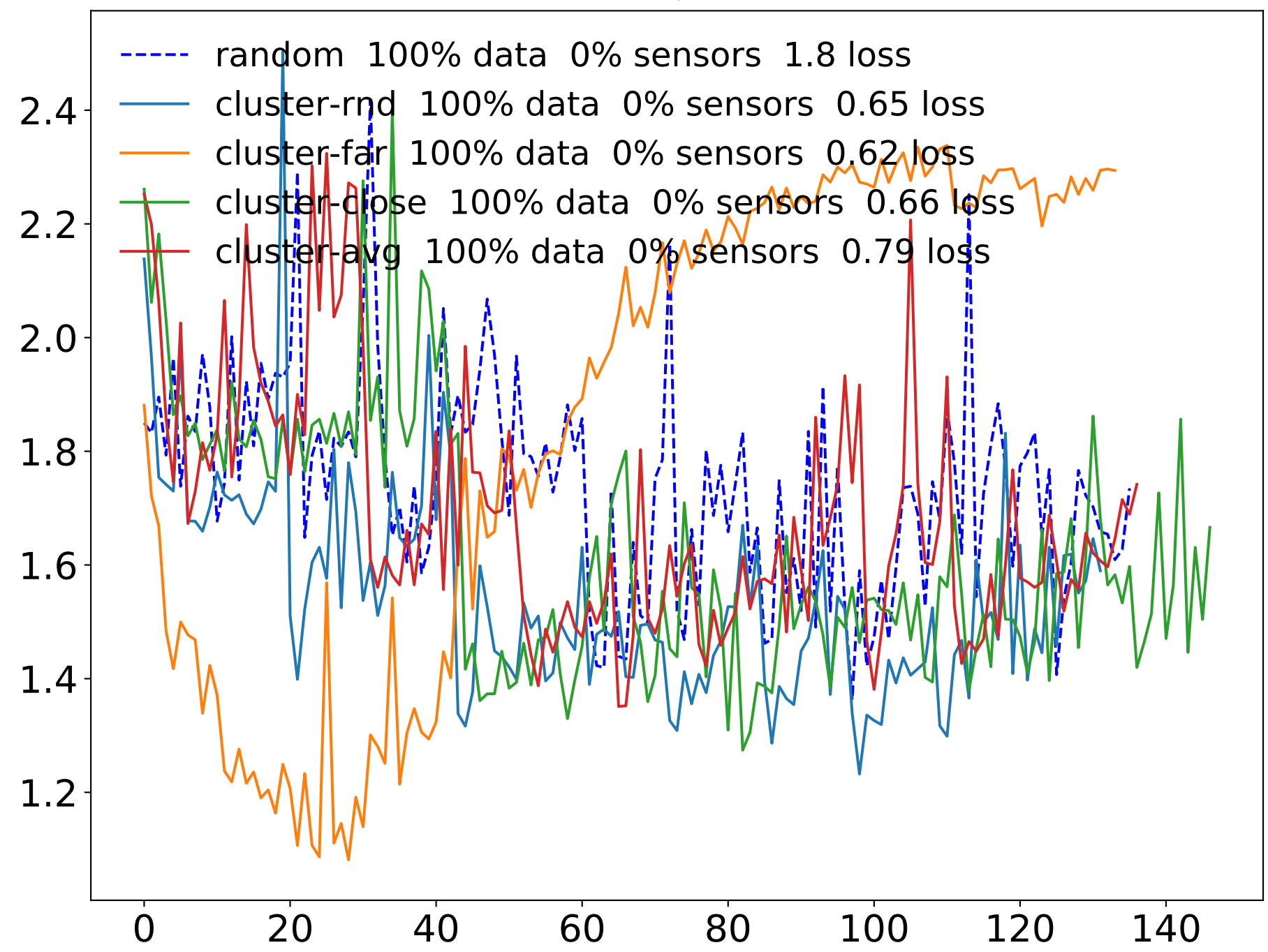
Validation losses
