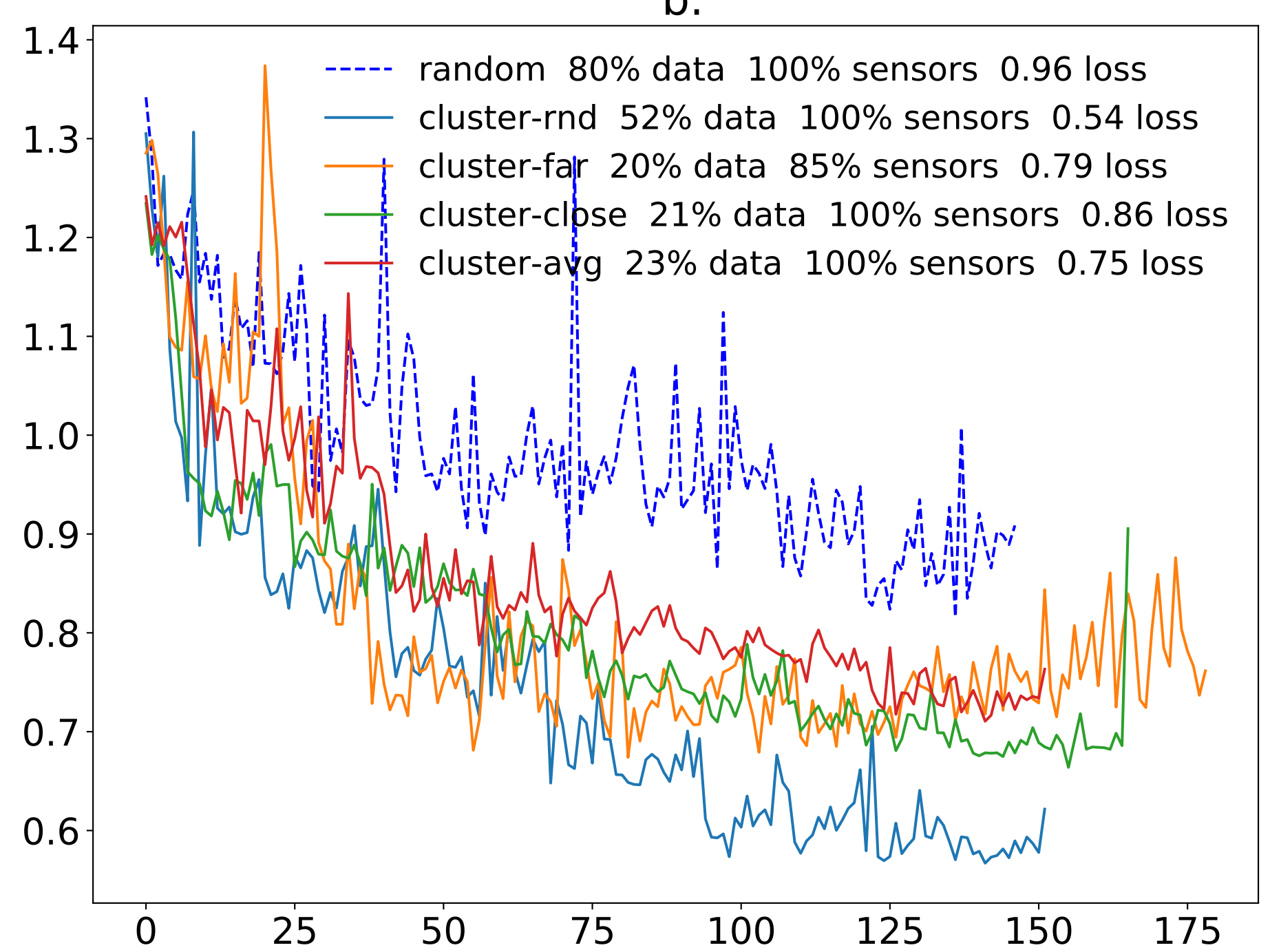
Validation losses
