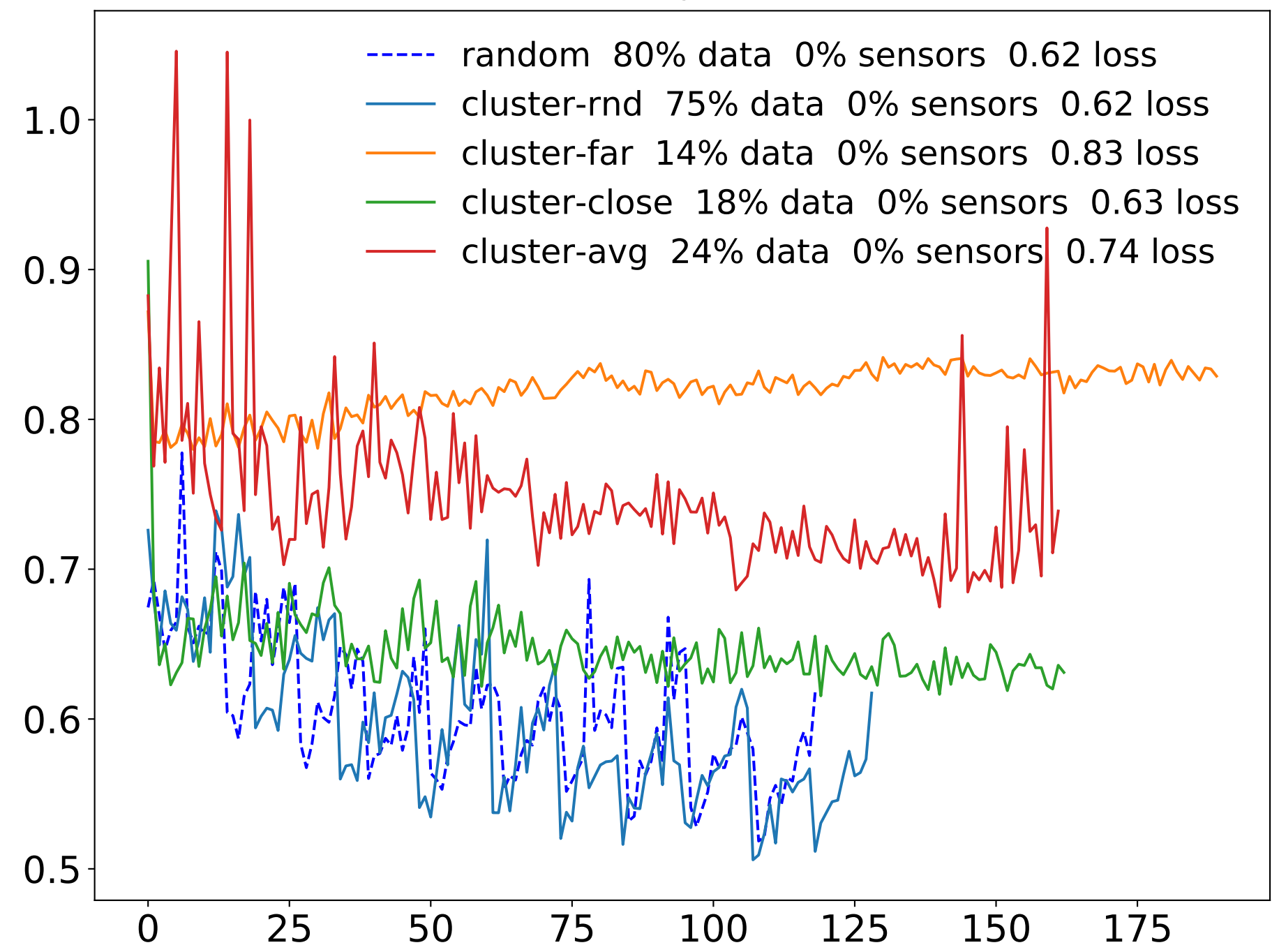
Validation losses
