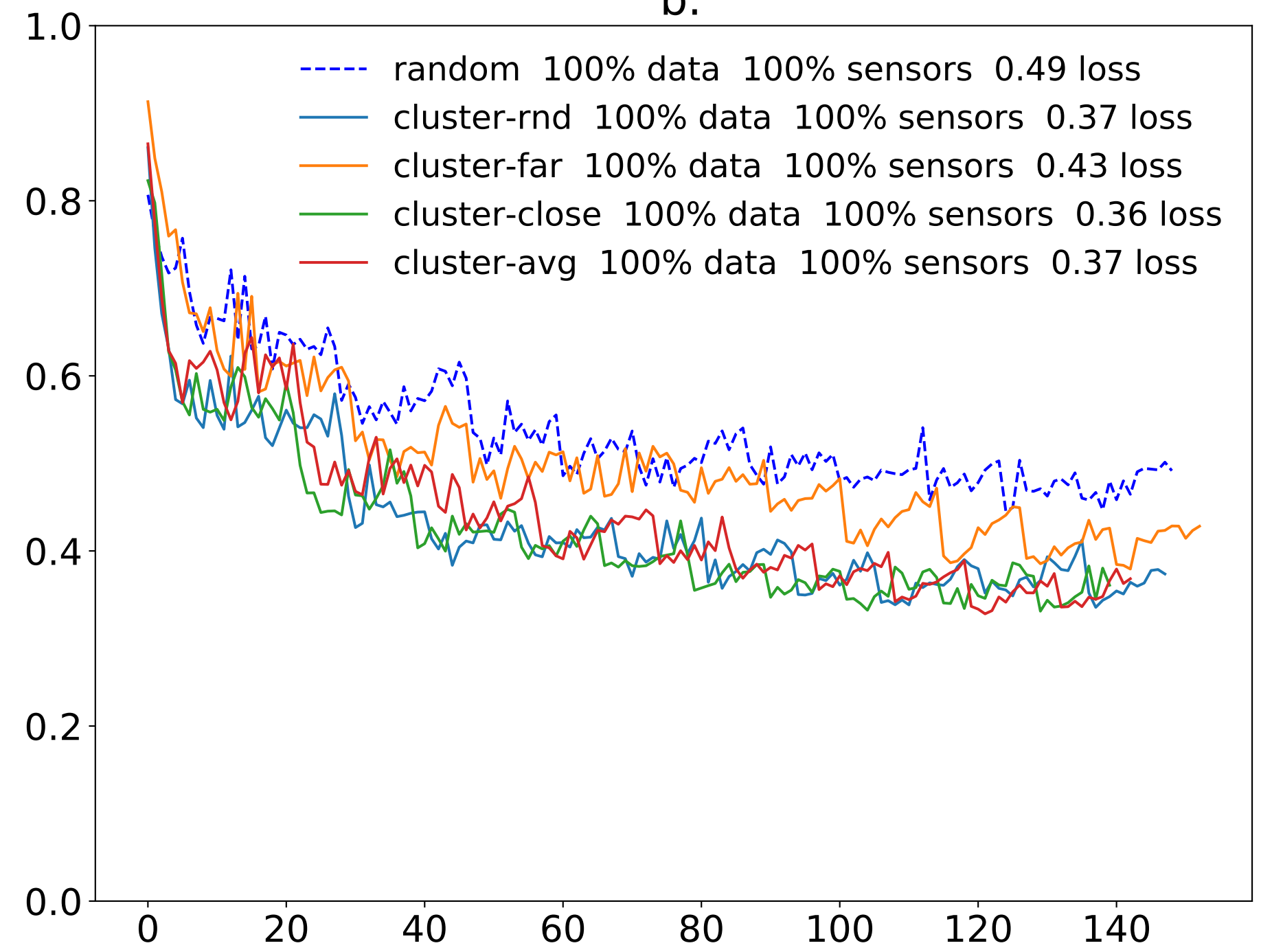
Validation losses
