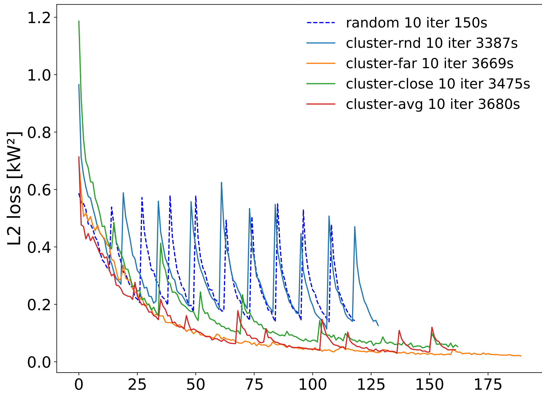
Training losses
