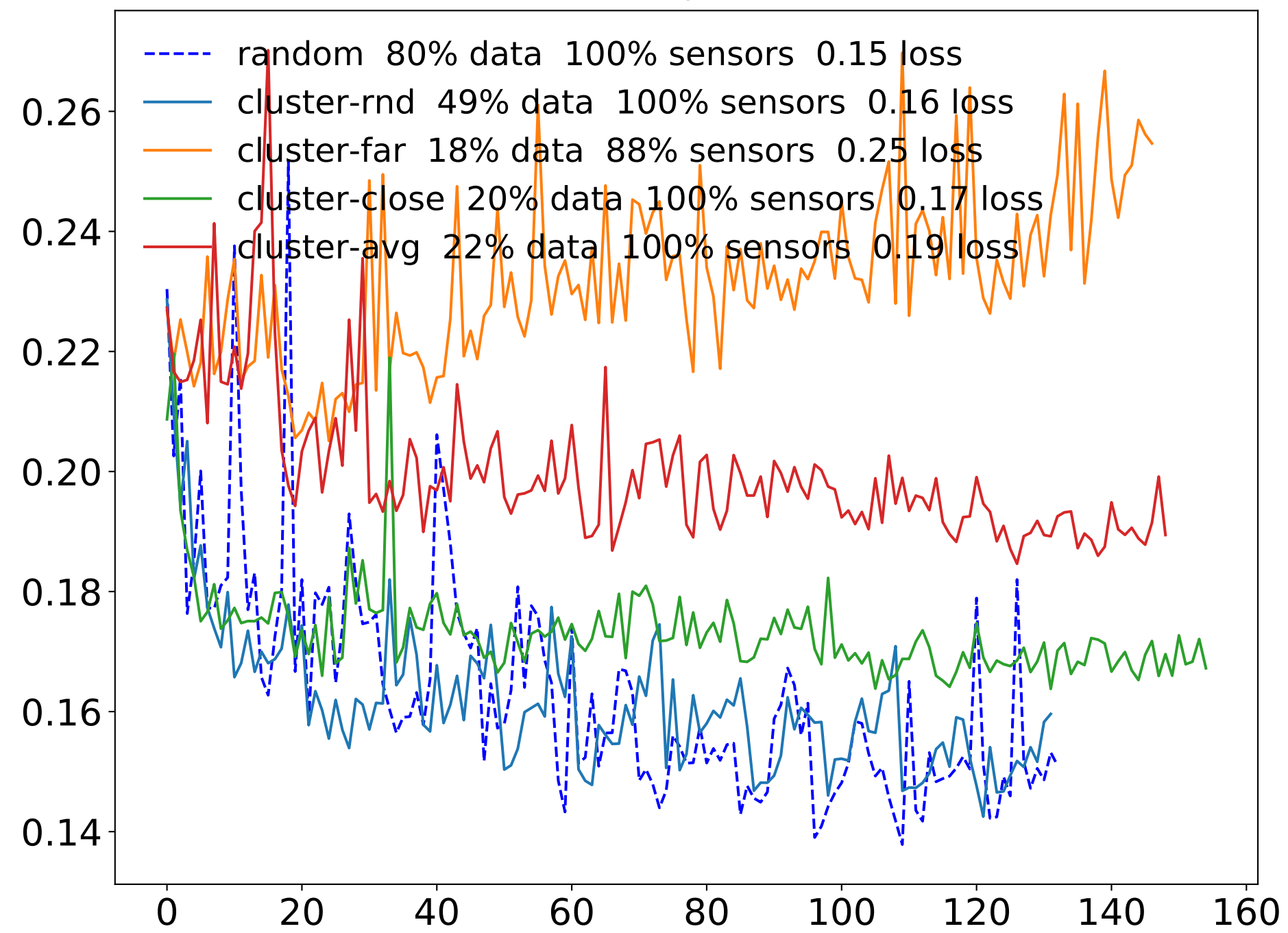
Validation losses
