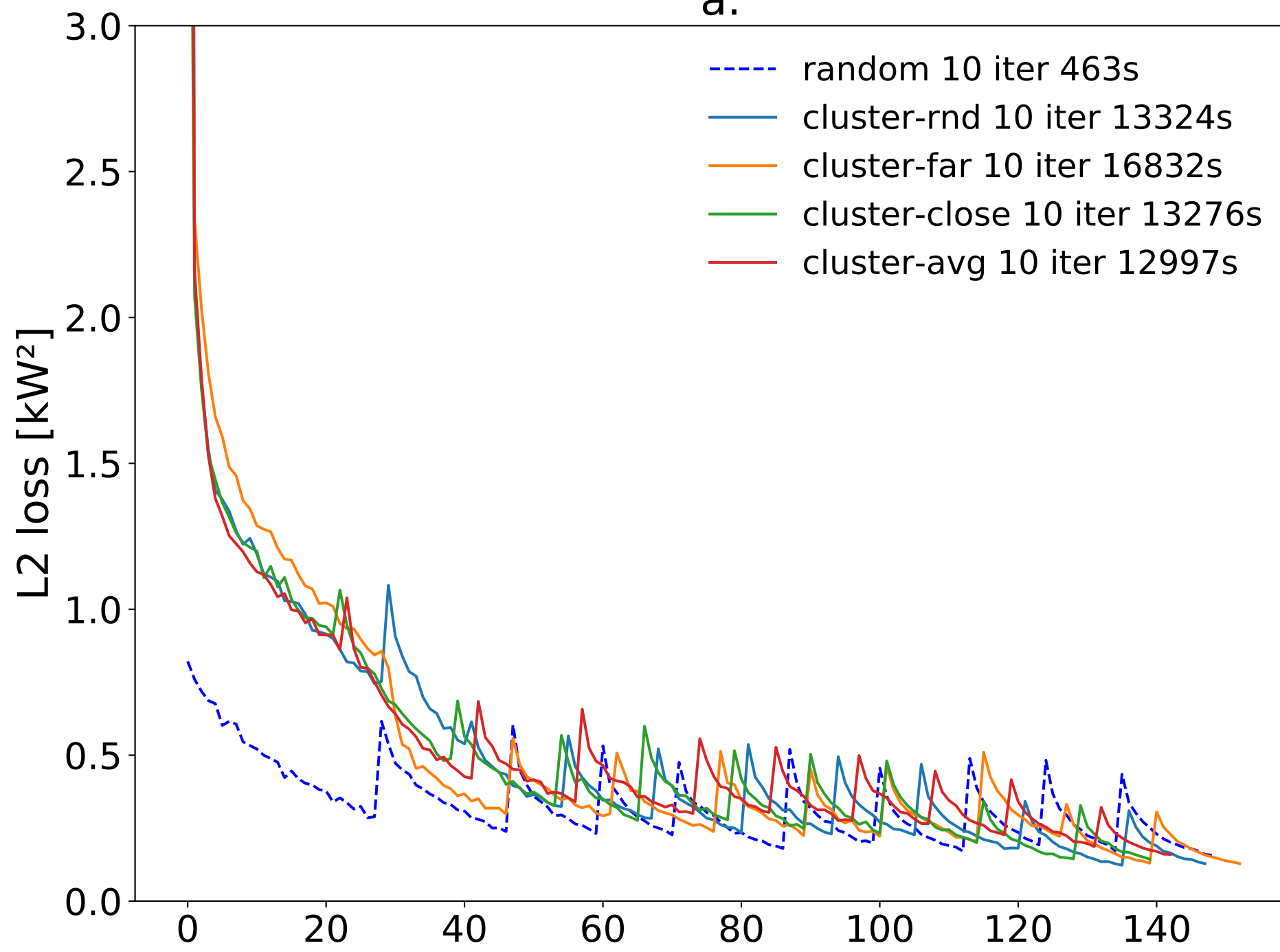
Training losses
