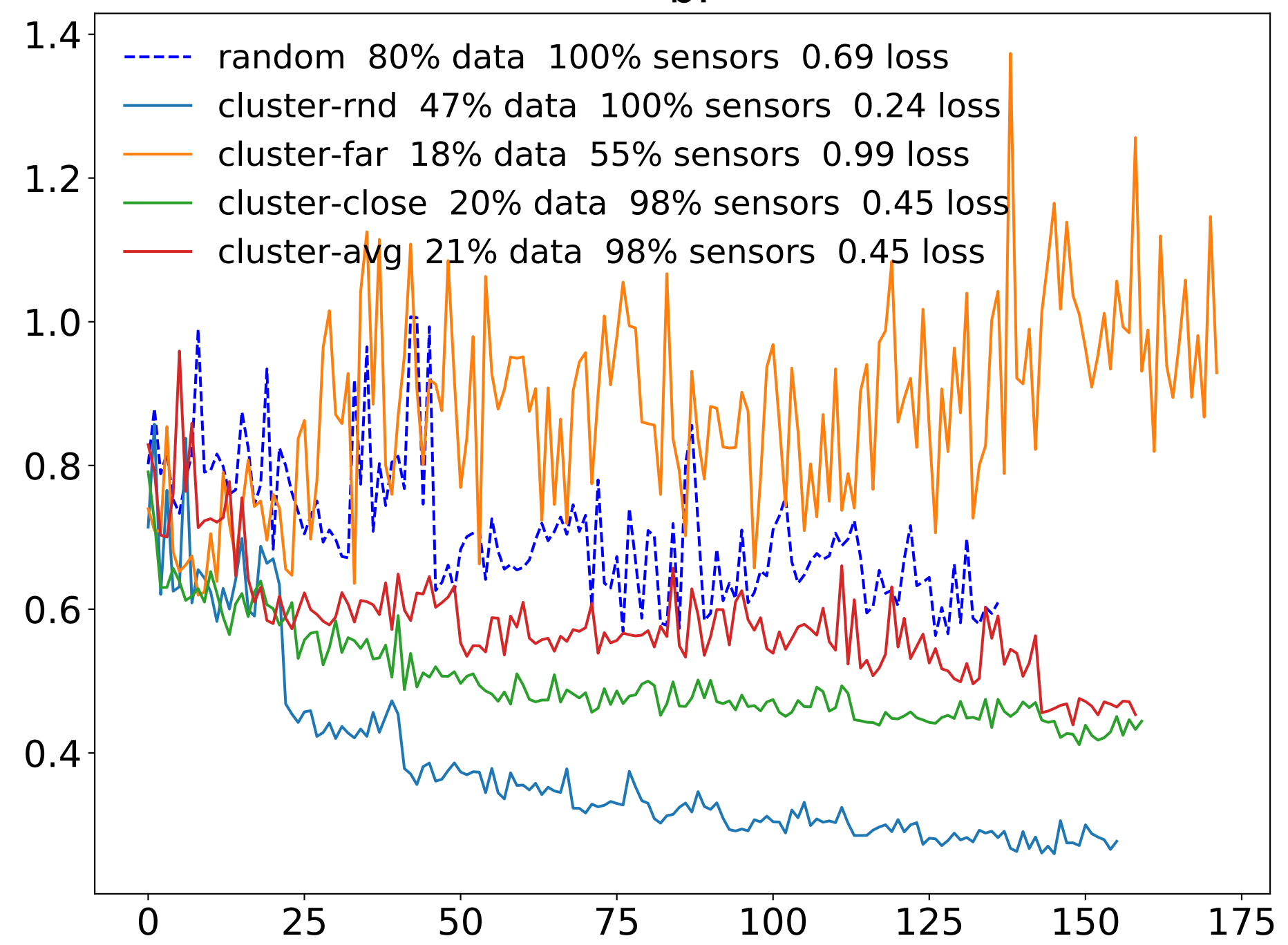
Validation losses
