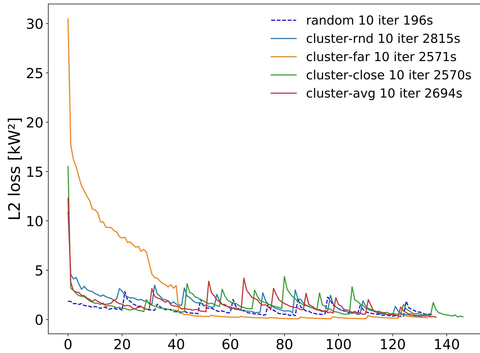
Training losses
