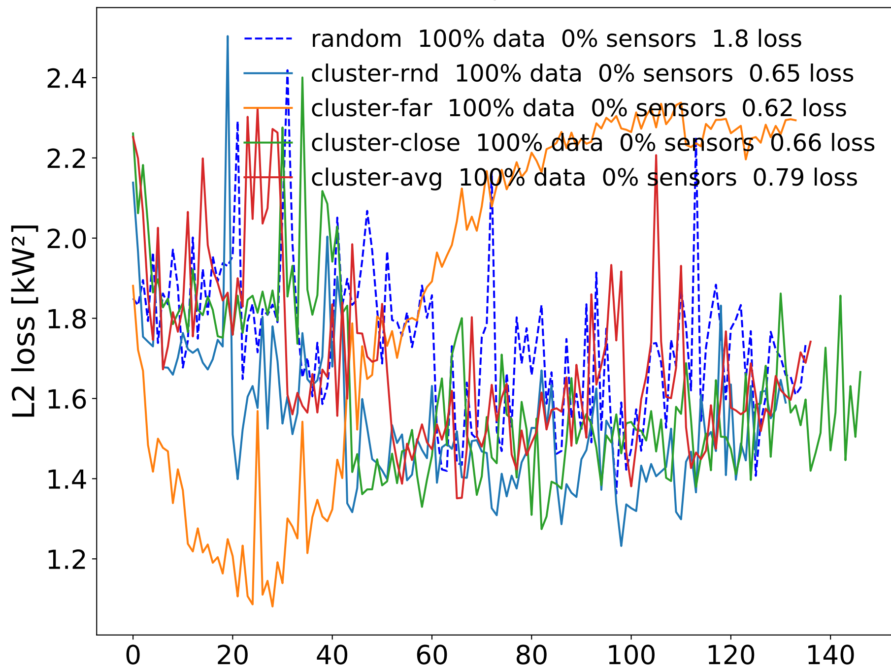
Validation losses with \delta=1
