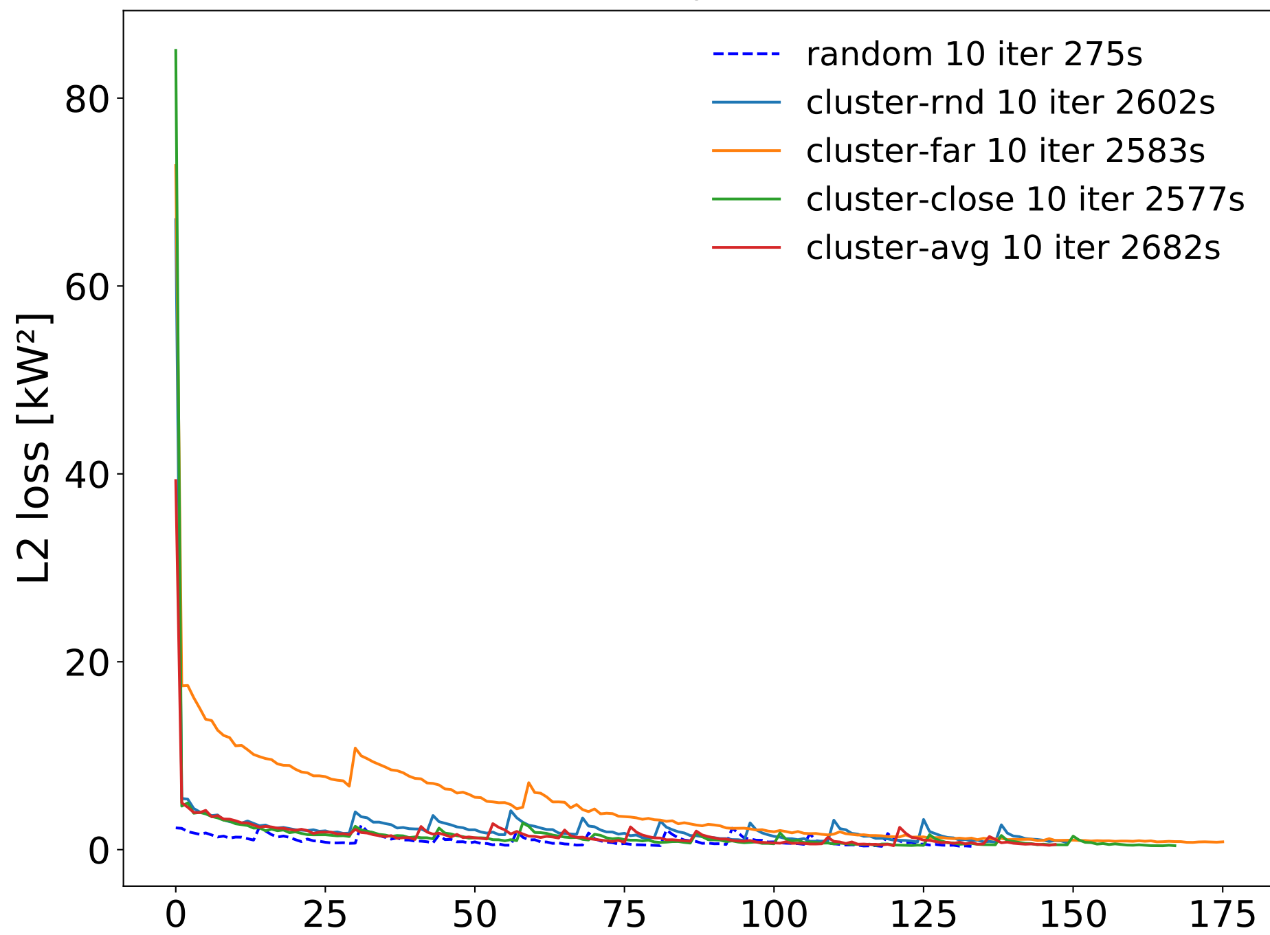
Training losses
