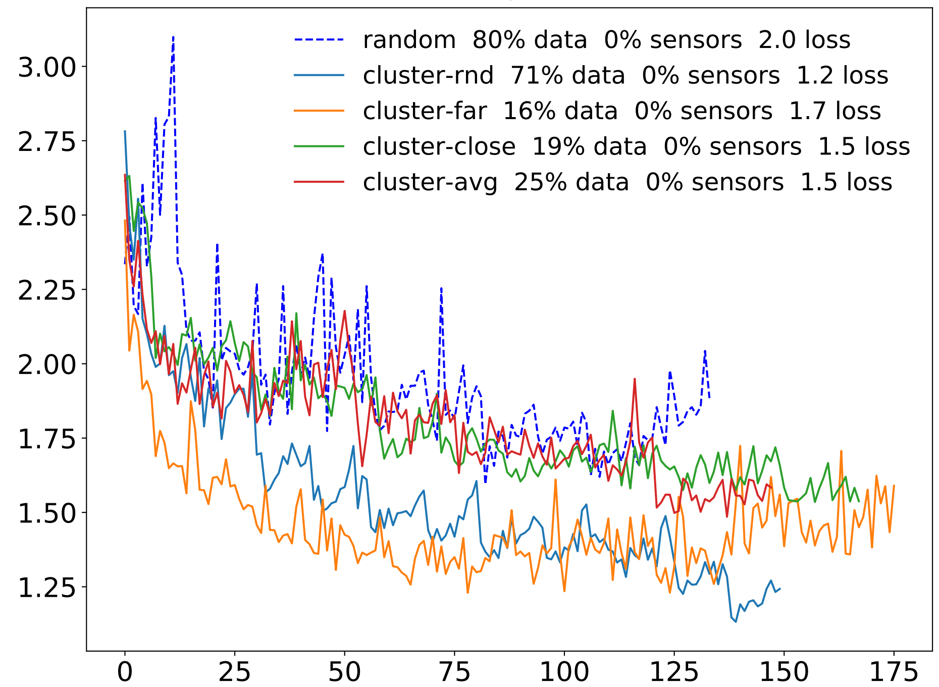
Validation losses
