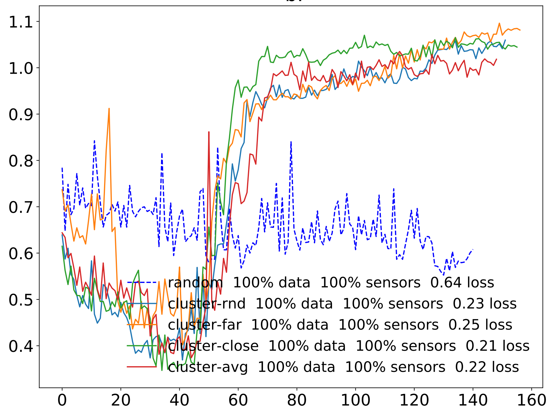
Validation losses
