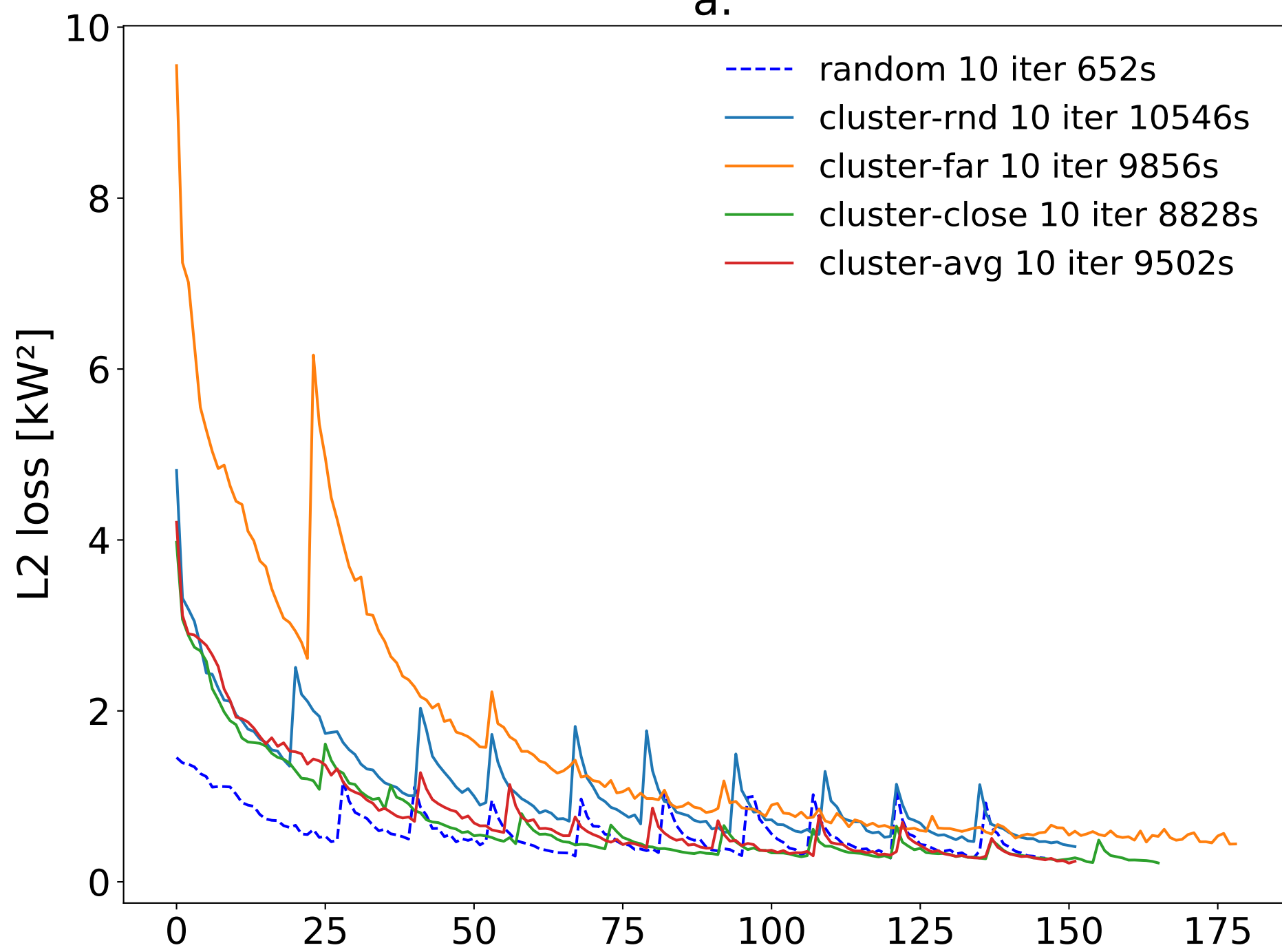
Training losses
