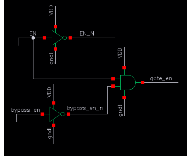
Figure 11. Enable Signal Logic Implementation
