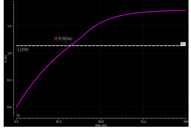
Figure 10. Finding the Parasitic Capacitance at the Gate of the Pass Transistor Through Simulation
