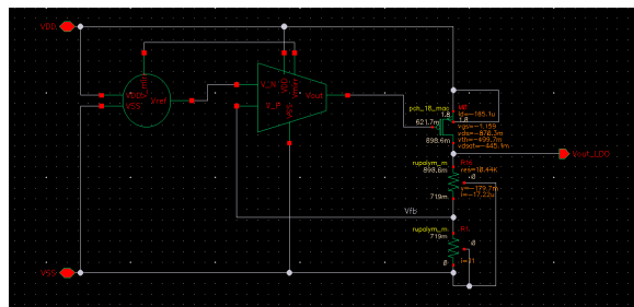
Figure 26. LDO schematic with annotated DC operating points.
