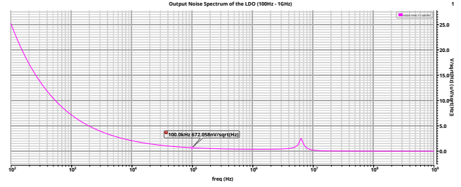
Figure 35. Post-layout output noise spectrum ( 100 Hz– 1 GHz).
