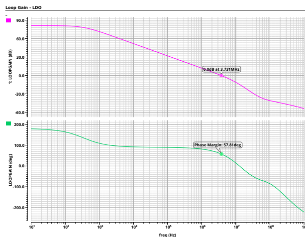
Figure 30. LDO loop gain and phase margin.
