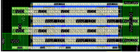
Figure 17. PMOS Pass Transistor Layout with Metal Stacking and Current Spreading
