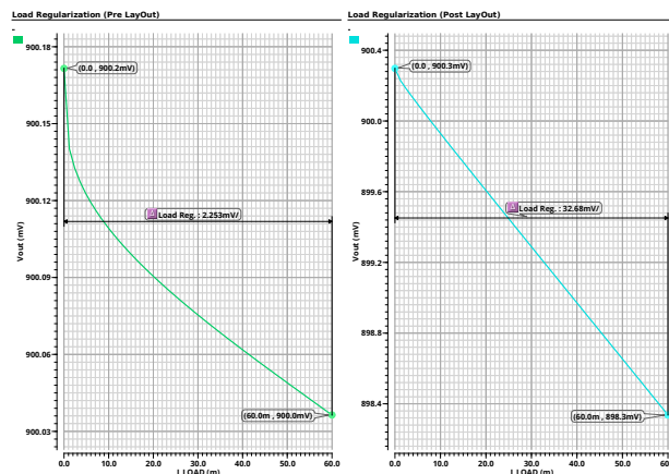
Figure 29. Pre- and post-layout load regulation.
