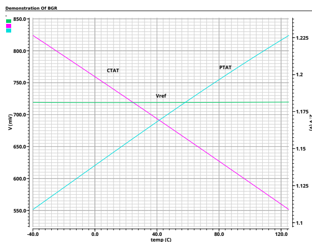
Figure 23. BGR concept: PTAT + CTAT \rightarrow near-zero TC V_{ref} .
