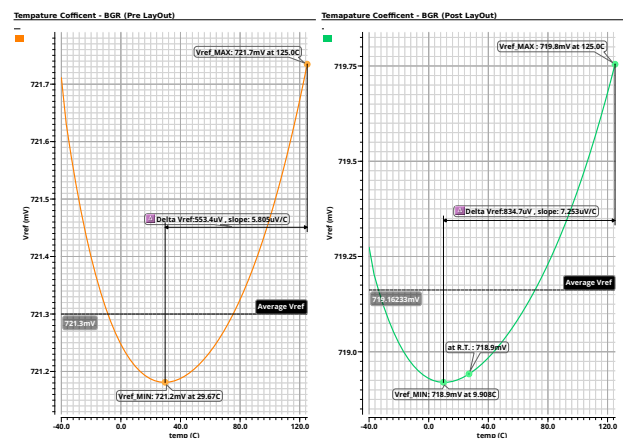
Figure 25. V_{\text{ref}} TC before/after layout.
