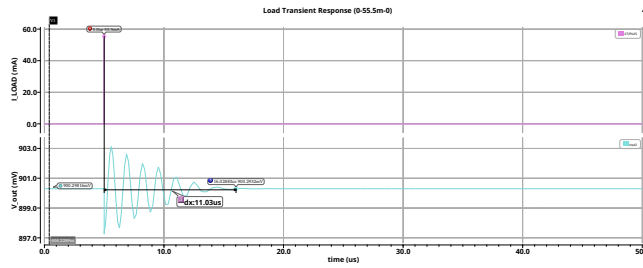
Figure 33. Post-layout transient response with 5 m \Omega output resistor.
