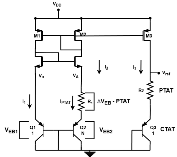
Figure 9. Current-Mirror Based BGR Topology
