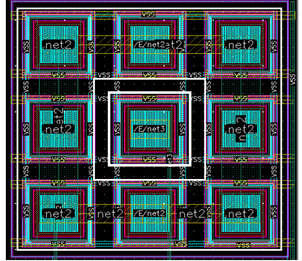
Figure 15. Common-Centroid Layout of Diode-Connected PNP Transistors
