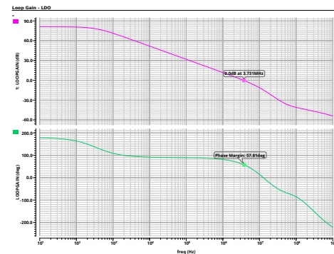
Figure 35. LDO Loop Gain and Phase Margin
