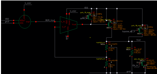
Figure 44. Normal operation DC operating point.
