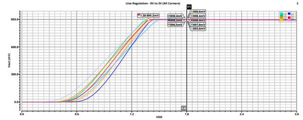
Figure 41. Line regulation across PVT corners
