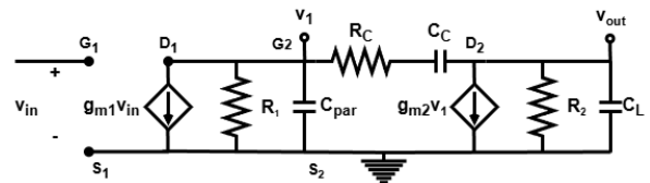
Figure 7. Small-Signal Model of the Two-Stage Miller OTA
