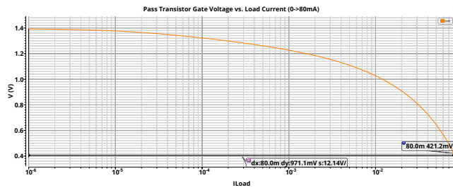
Figure 31. Gate modulation of pass transistor in response to load change
