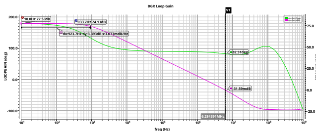
Figure 25. BGR loop gain simulation
