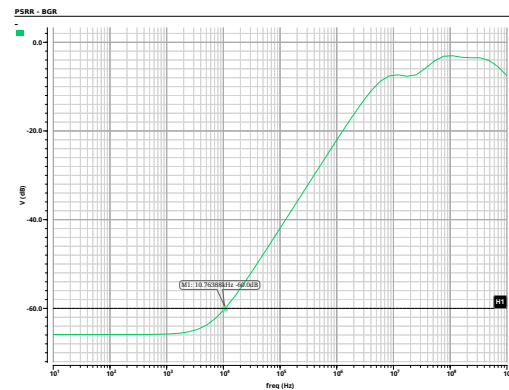
Figure 28. PSRR of the Bandgap Reference Block
