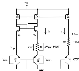
Figure 10. Current-Mirror Based BGR Topology
