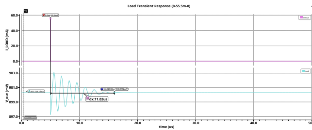
Figure 38. Post-layout transient response with 5 m \Omega output resistor
