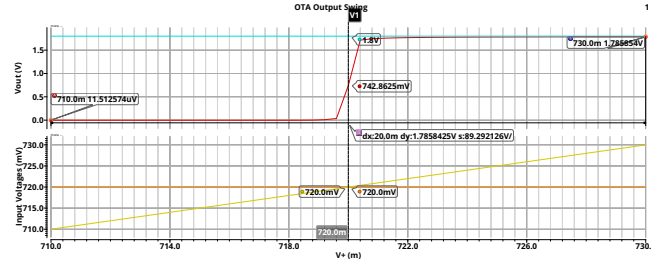
Figure 22. Output swing of the OTA, showing near rail-to-rail behavior.
