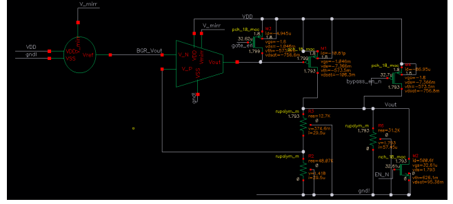
Figure 45. Bypass mode DC operating point.
