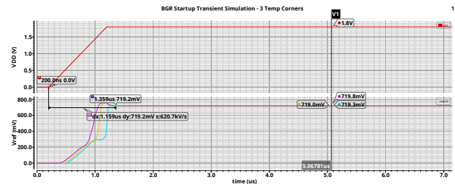
Figure 29. Startup Behavior of the BGR
