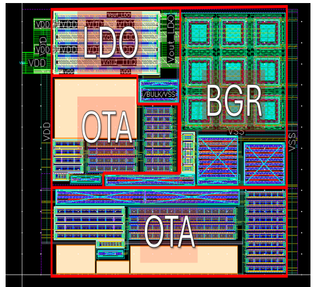
Figure 19. Final Integrated Layout of OTA, Bandgap Reference, and LDO
