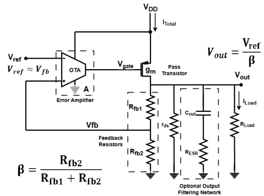
Figure 3. LDO Circuit for Line/Load Regulation and Stability Analysis
