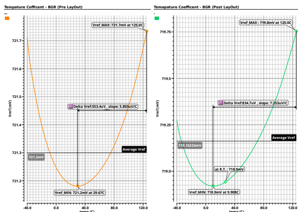
Figure 26. V_{ref} TC before/after layout
