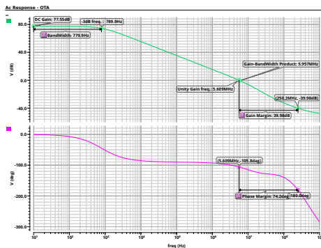
Figure 21. Open-loop AC response of the OTA.
