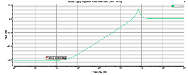
Figure 39. Post-layout PSRR ( 10 Hz– 1 GHz), V_{DD} = 1.8 V, I_{Load} = 55.5 mA
