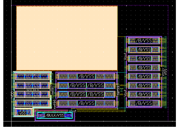
Figure 17. Modified OTA Layout for LDO: Compact and Square with Shared Biasing
