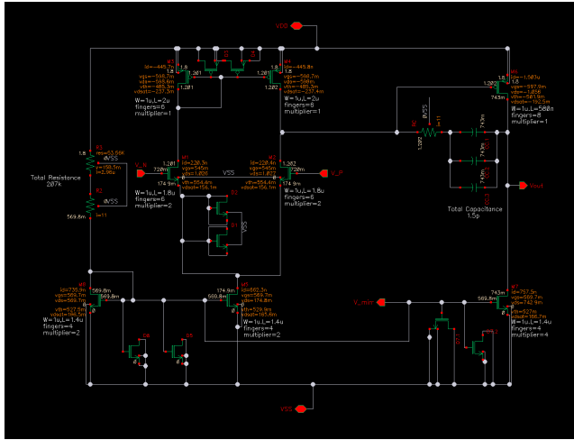
Figure 20. Post-layout DC operating point of the OTA.
