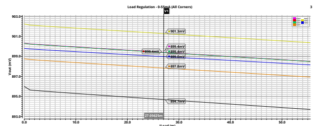
Figure 42. Load regulation across PVT corners
