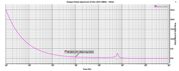
Figure 40. Post-layout output noise spectrum ( 100 Hz– 1 GHz)
