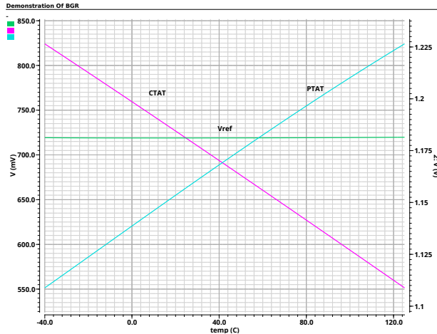
Figure 24. BGR concept: PTAT + CTAT → near-zero TC V_{ref}
