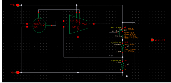
Figure 30. LDO schematic with annotated DC operating points
