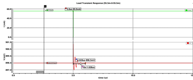
Figure 37. Post-layout transient response ( 55.5 mA \rightarrow 0 mA \rightarrow 55.5 mA)
