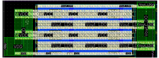
Figure 18. PMOS Pass Transistor Layout with Metal Stacking and Current Spreading
