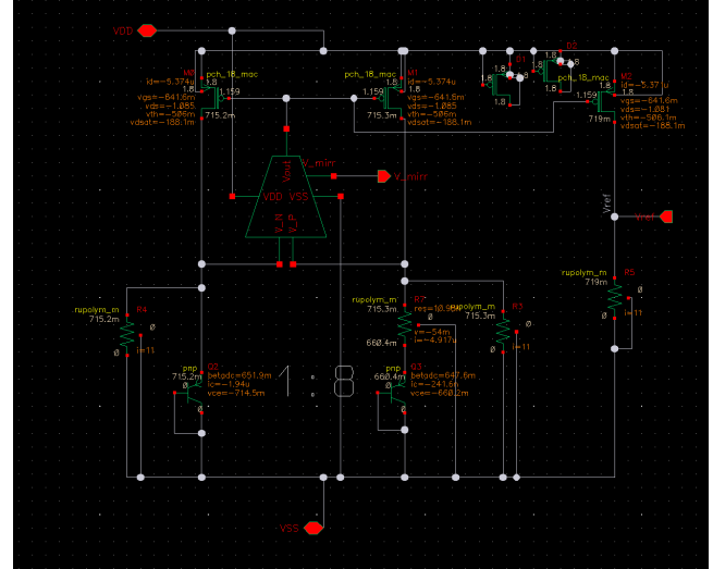
Figure 23. BGR schematic with annotated operating points
