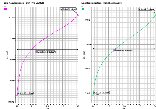
Figure 27. Line Regulation of V_{ref} before/after layout
