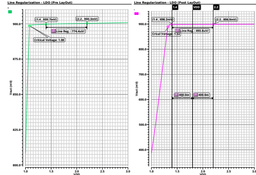
Figure 33. Pre- and Post-Layout Line Regulation
