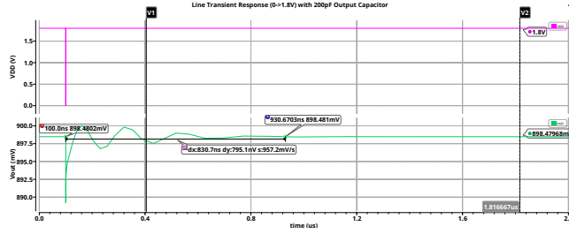
Figure 36. Transient response with 200 pF output capacitance
