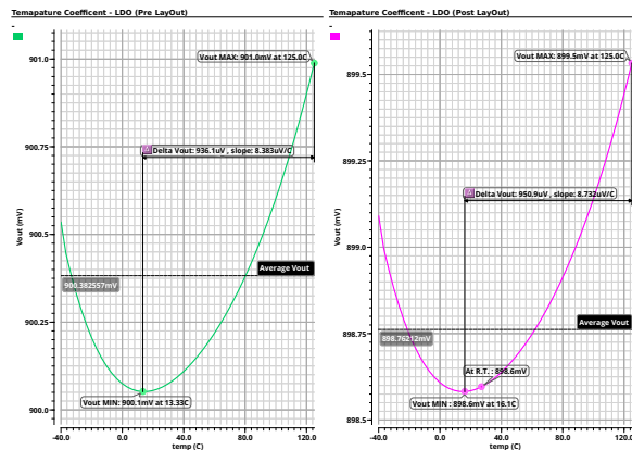
Figure 32. Pre- and Post-Layout LDO TC
