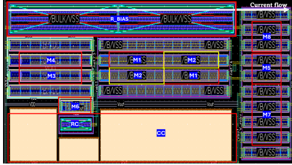
Figure 15. OTA Floorplan showing Functional Block Arrangement
