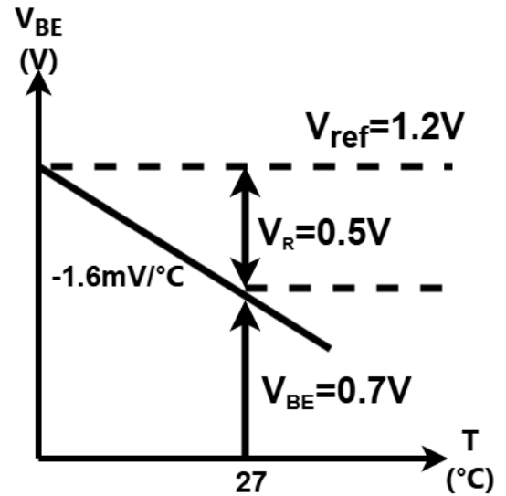
Figure 8. Temperature Compensation in a Bandgap Reference: Combining CTAT and PTAT Components to achieve a stable \sim 1.2\text{ V} output.
