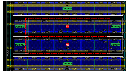
Figure 13. Layout of M3 and M4 with Dummy Devices and Symmetric Routing
