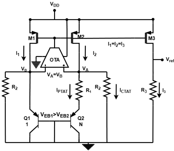
Figure 9. Current-Mode Bandgap Reference Circuit Topology
