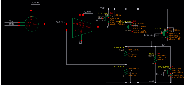
Figure 43. Disabled mode DC operating point.
