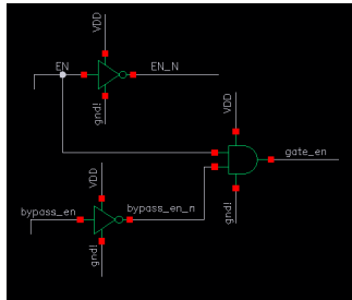
Figure 12. Enable Signal Logic Implementation
