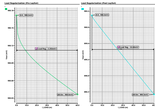
Figure 34. Pre- and Post-Layout Load Regulation
