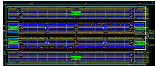
Figure 14. Common-Centroid Layout of Differential Pair with Symmetric H-shaped Routing
