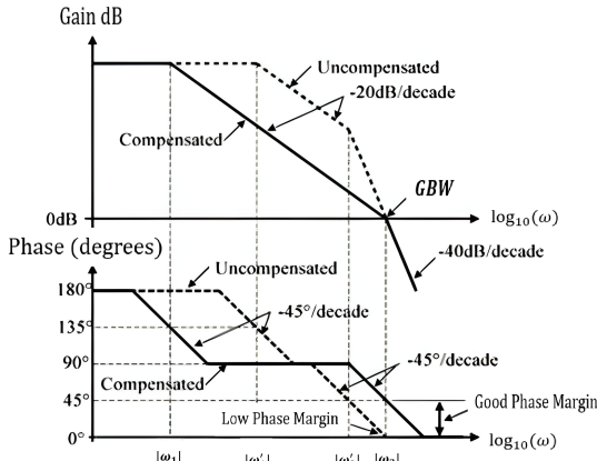
Figure 5. Bode Plot: Compensated vs. Non-compensated OTA
