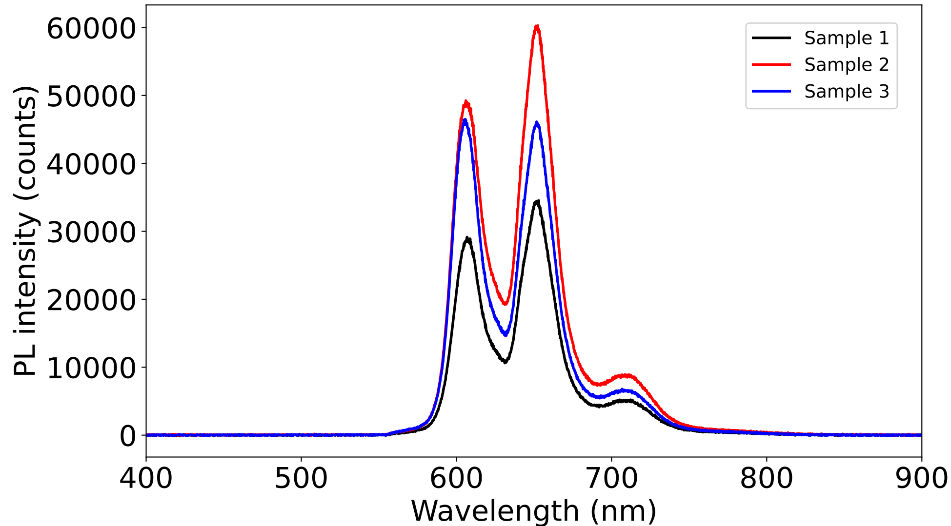
PL of 3 Samples Made from a PTP/PC Melt (10ms)
