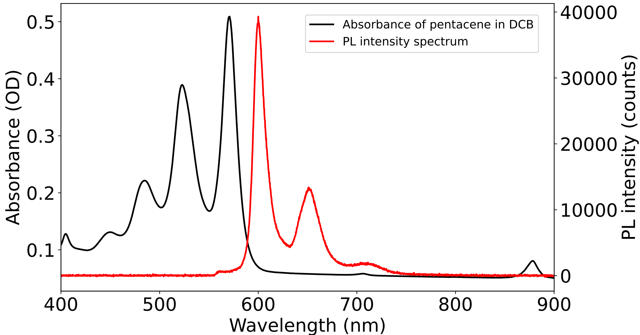
Absorbance and PL intensity of sample #5
