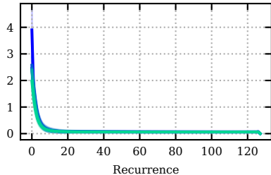
Retrofitted Llama (128 steps)
