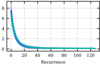
Huginn-0125 (128 steps)
