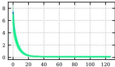
Huginn-0125 (128 steps)
