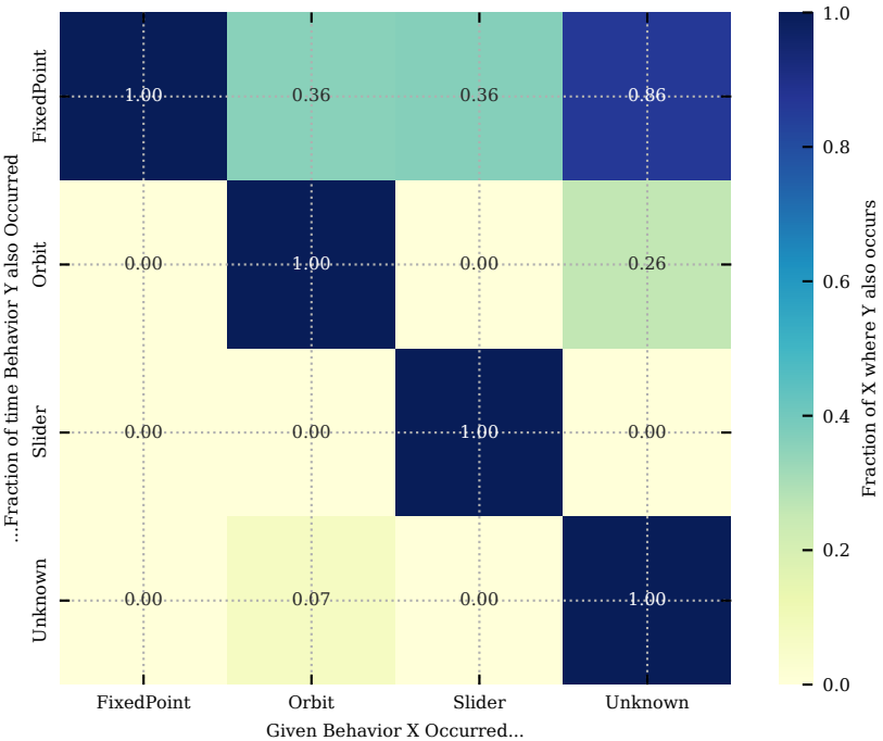
Conditional Behavior Co-occurrence: P(Y | X)
