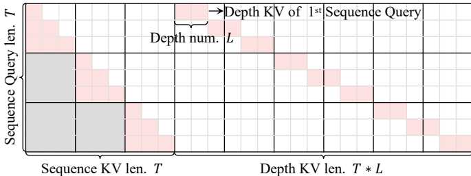
Flash-Compatible Hardware-Efficient MoDA
