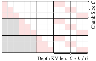
Chunk/Group-Aware MoDA
