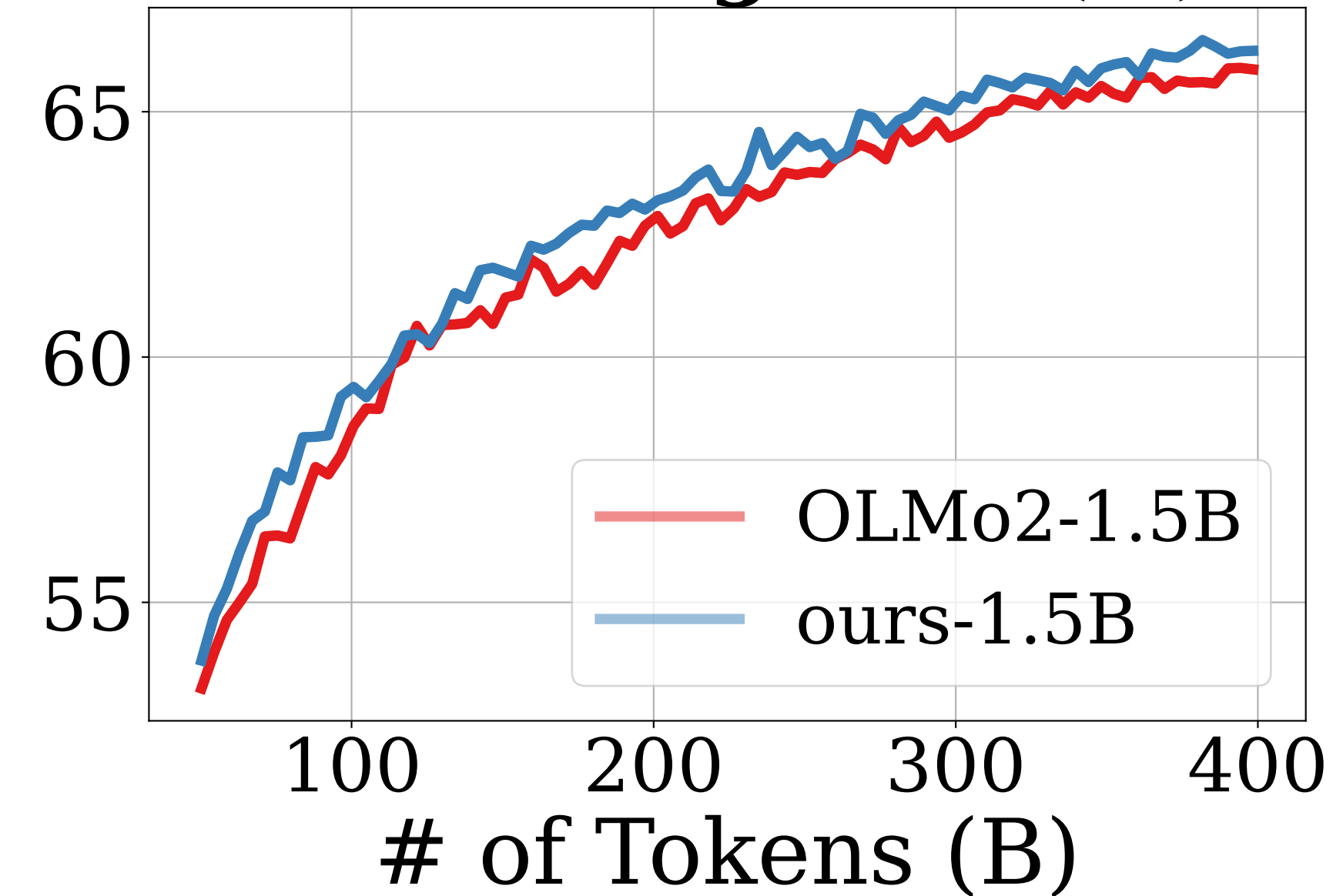
HellaSwag Acc. (%)
