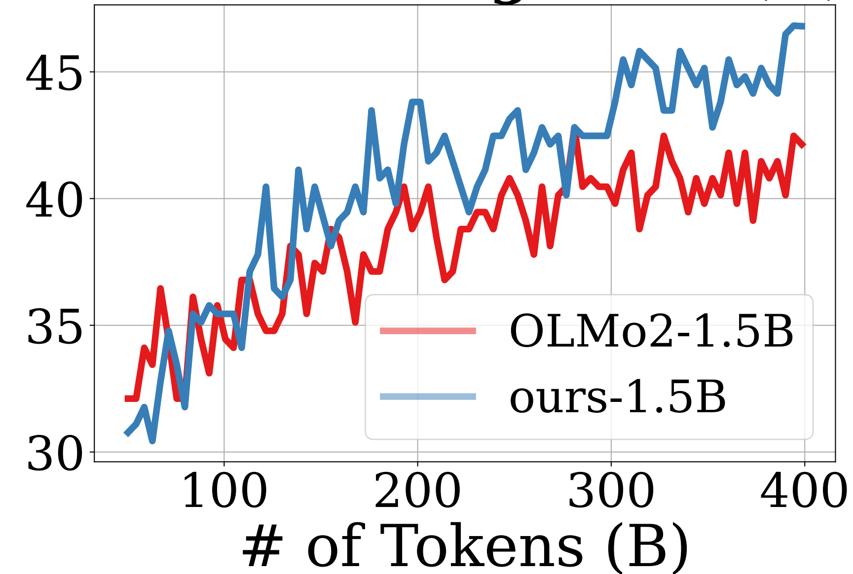
ARC-Challenge Acc. (%)
