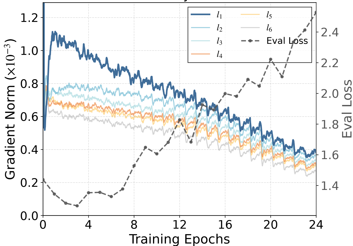
Gradient Norms by Latent Position
