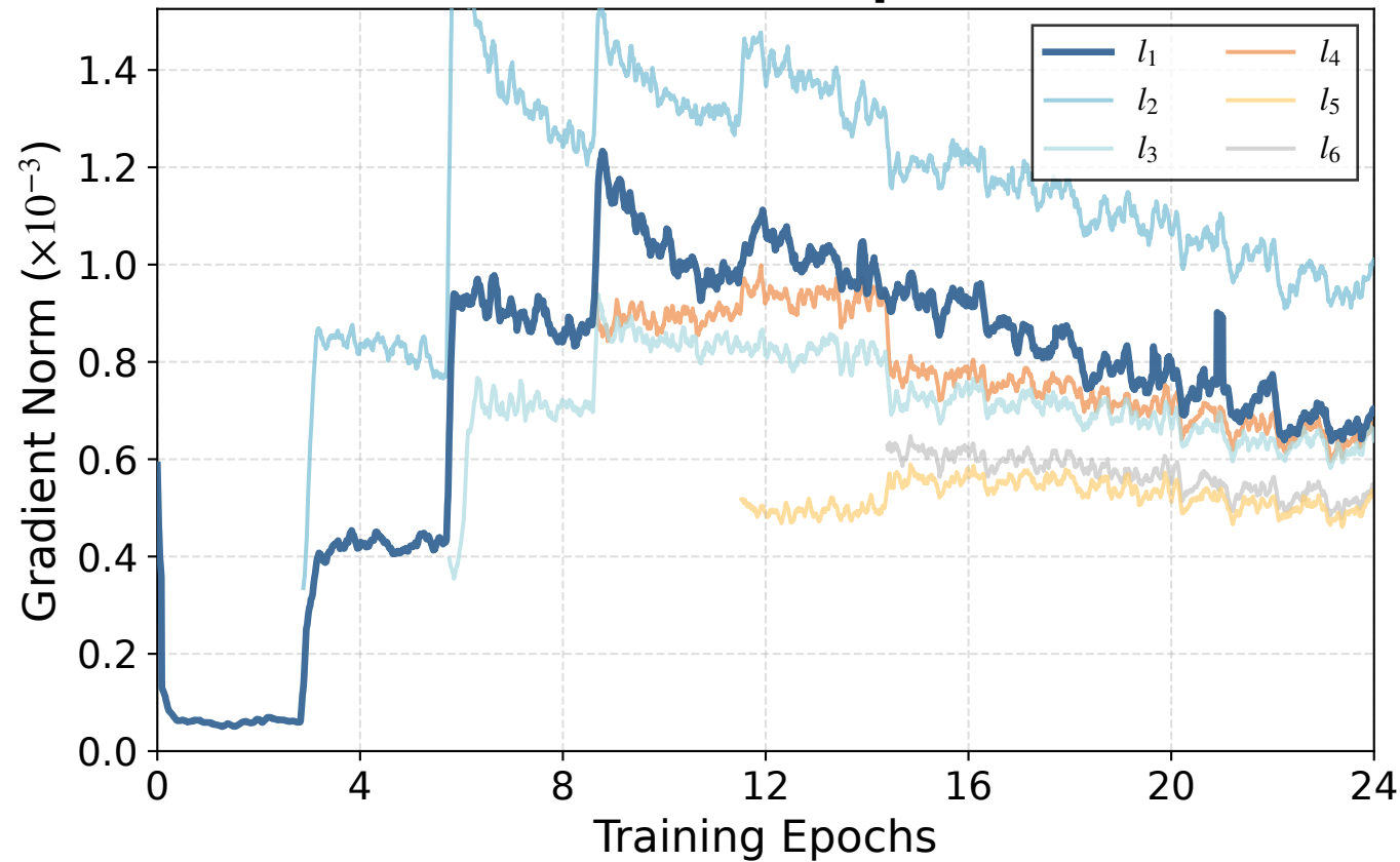
(a) With Reset Optimizer
