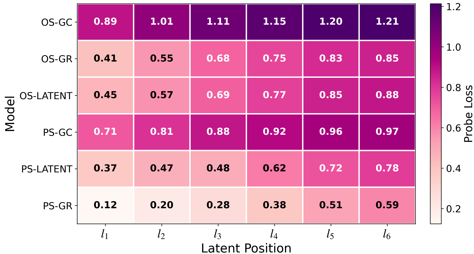
Per-Latent Probe Reconstruction Loss
