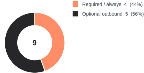
Network flows
