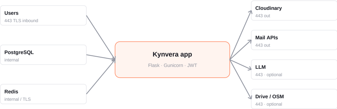
Network flows
