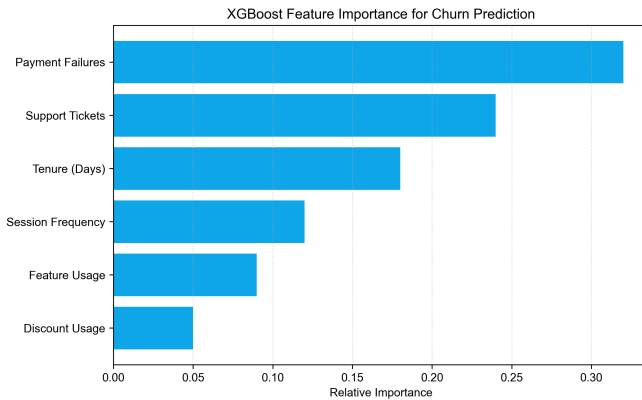
Fig. 7. Relative feature importance generated by the XGBoost model.
