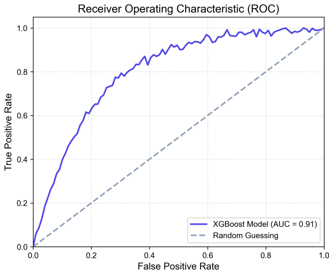
Fig. 6. Receiver Operating Characteristic (ROC) curve for the XGBoost churn prediction model.
