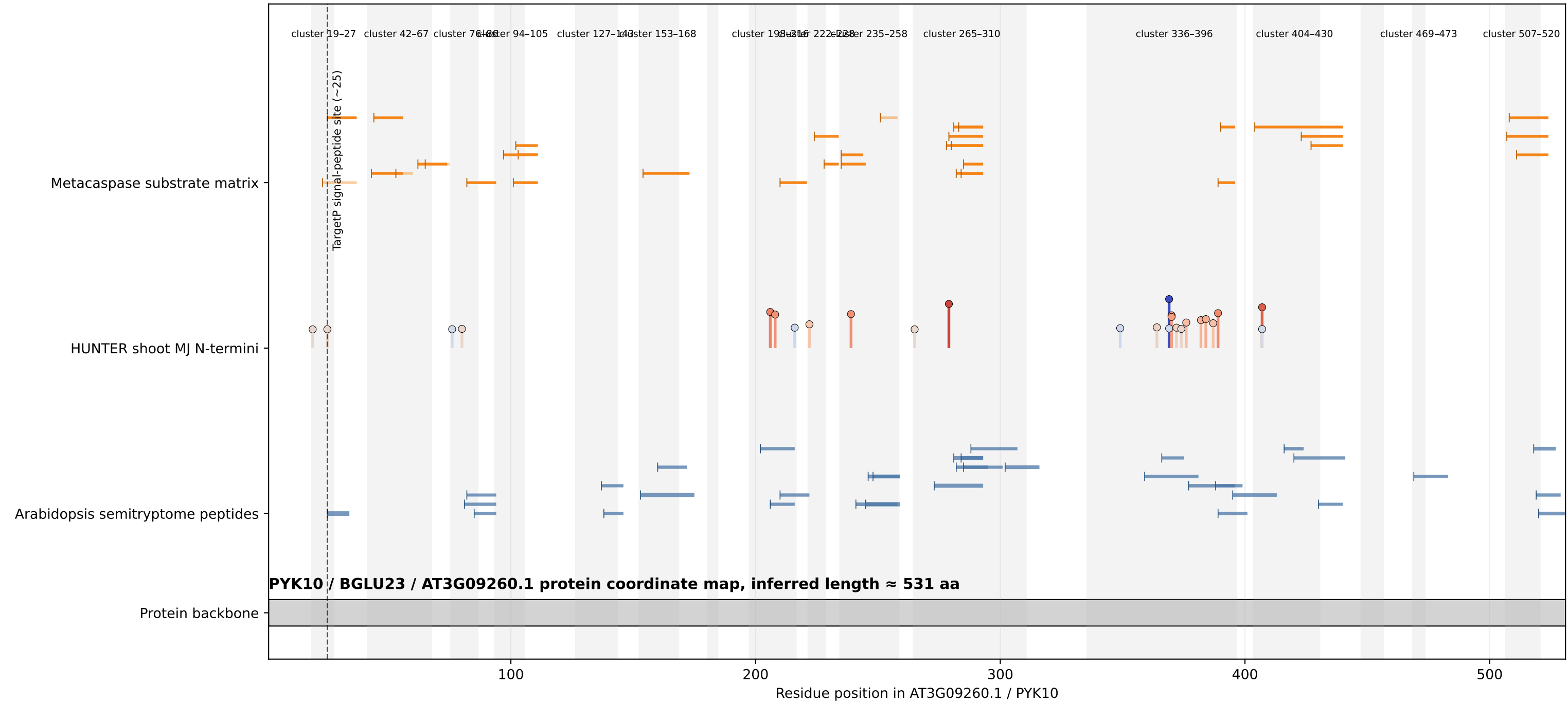
Integrated peptide coverage and cleavage-site evidence for Arabidopsis PYK10
