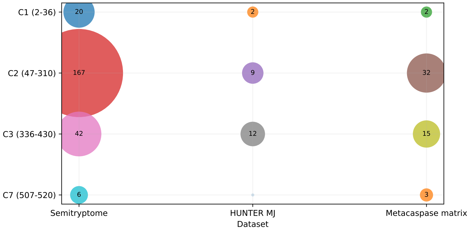
AT3G09260.1 cluster-level evidence matrix
