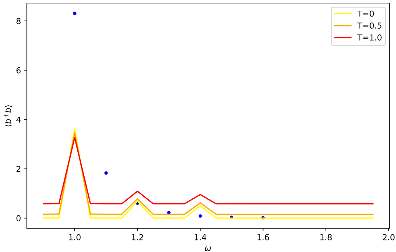
\langle b^\dagger b \rangle vs \omega
