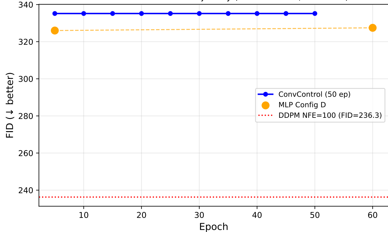
ConvControl vs MLP: FID Trajectory (FashionMNIST, NFE=100)
