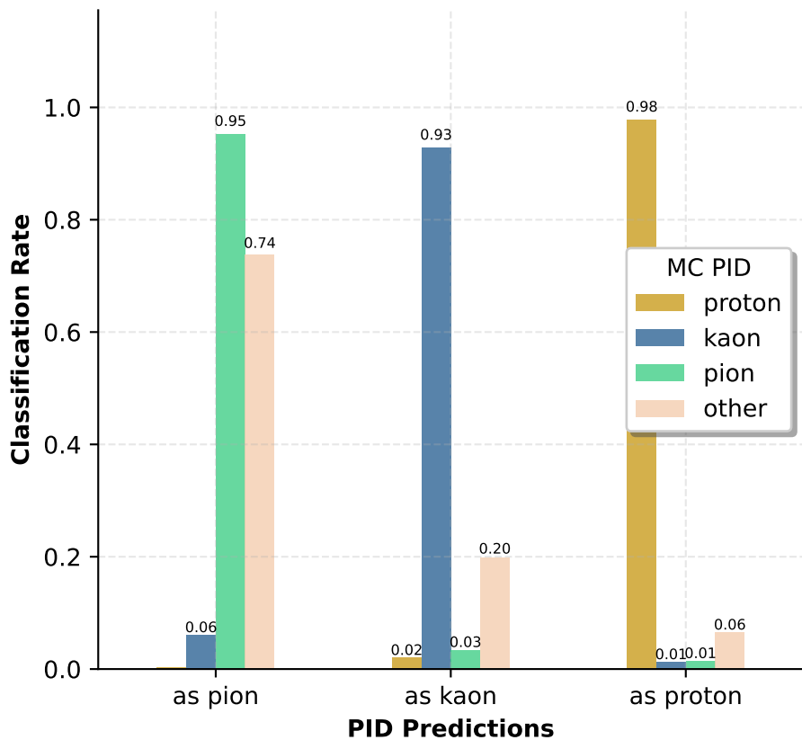
Classification Rate
