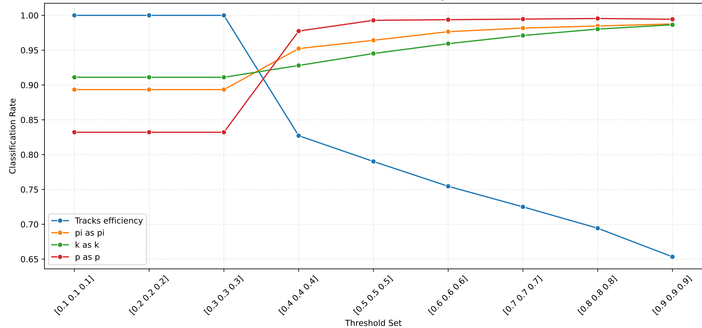
Classification Performance vs. Probability Thresholds
