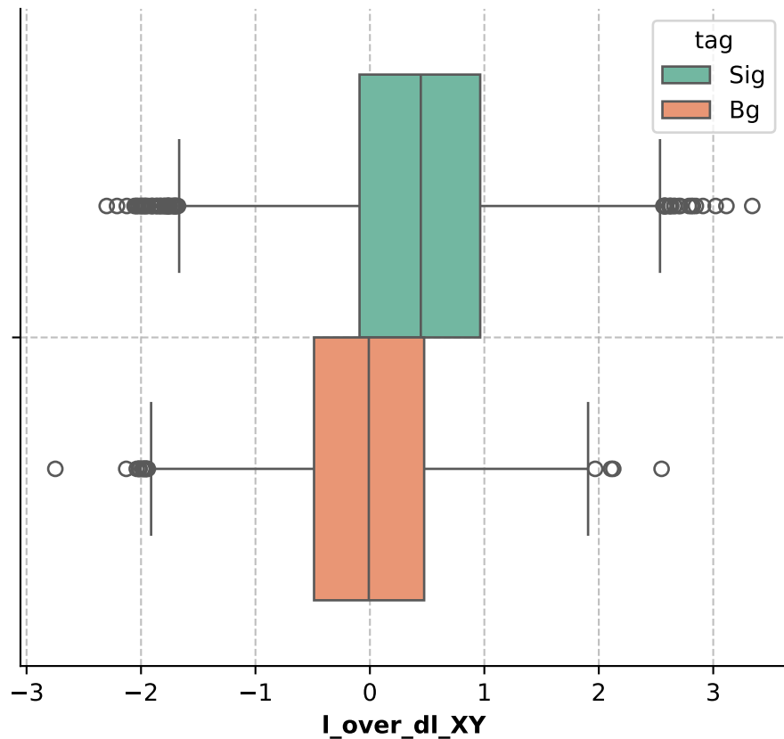
I_over_dl_XY Distribution
