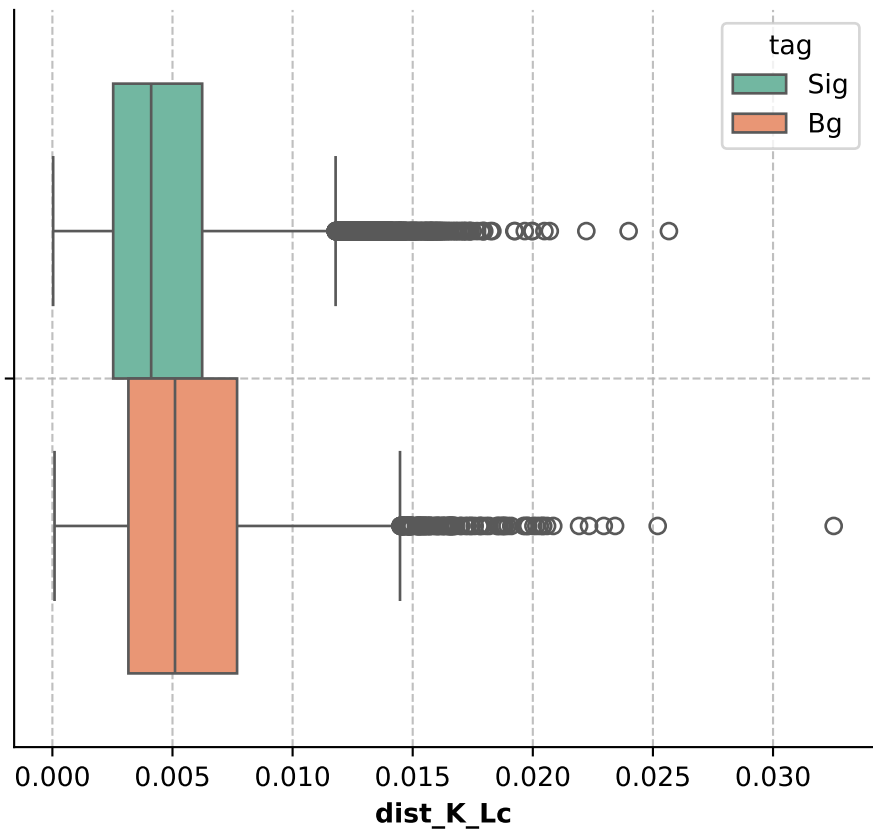
dist_K_Lc Distribution
