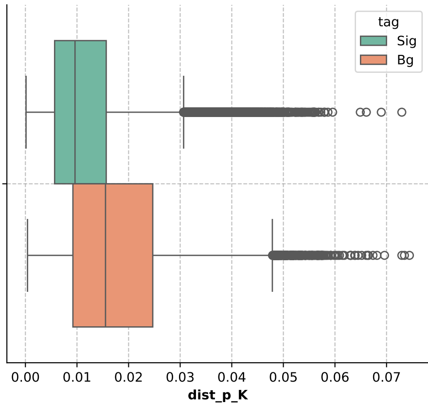
dist_p_K Distribution
