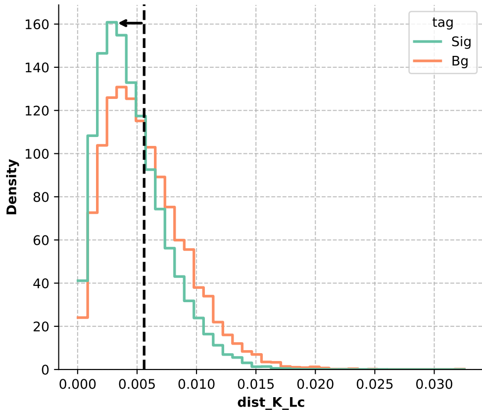
dist_K_Lc Distribution
