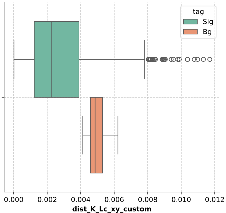
dist_K_Lc_xy_custom Distribution
