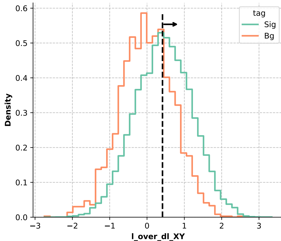
I_over_dl_XY Distribution
