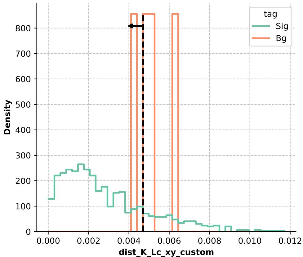
dist_K_Lc_xy_custom Distribution
