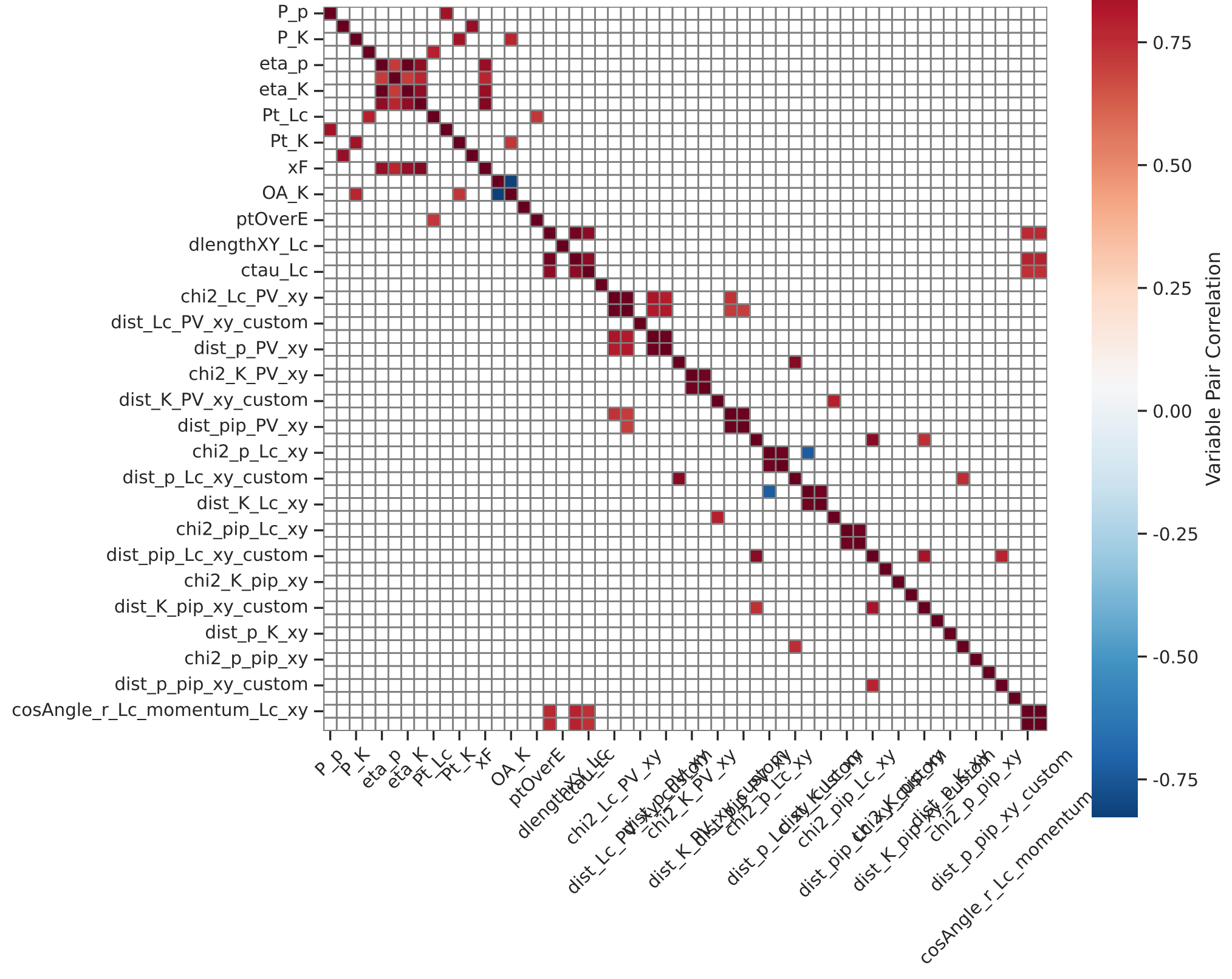
Signal Sample (abs(corr) > 0.7)
