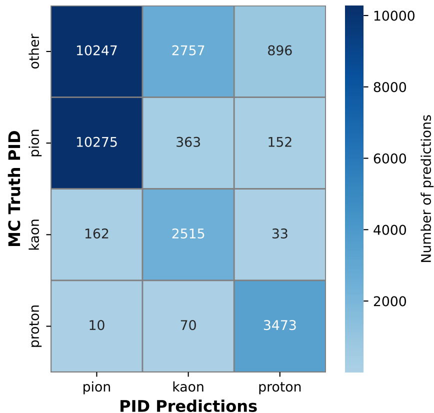
Confusion Matrix
