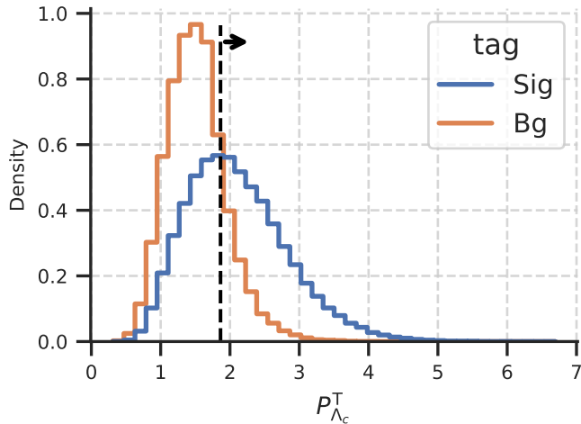
Feature Distribution
