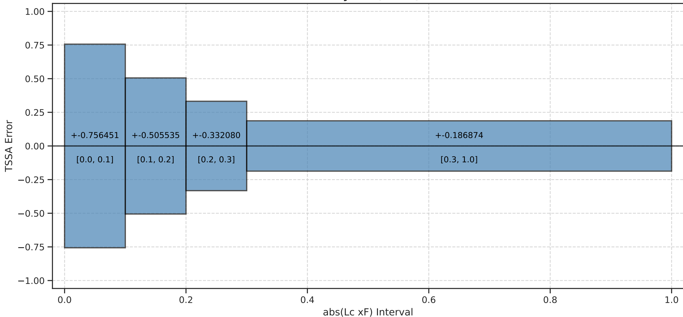
TSSA Error by abs(Lc xF) Interval
