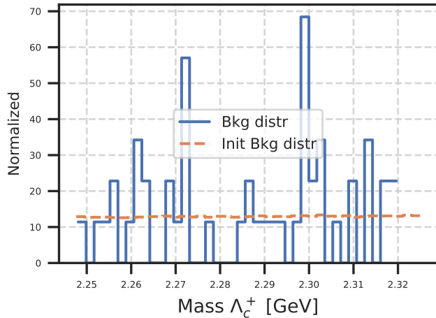
Background Distribution
