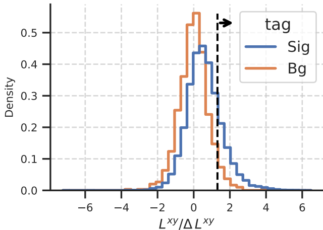
Feature Distribution
