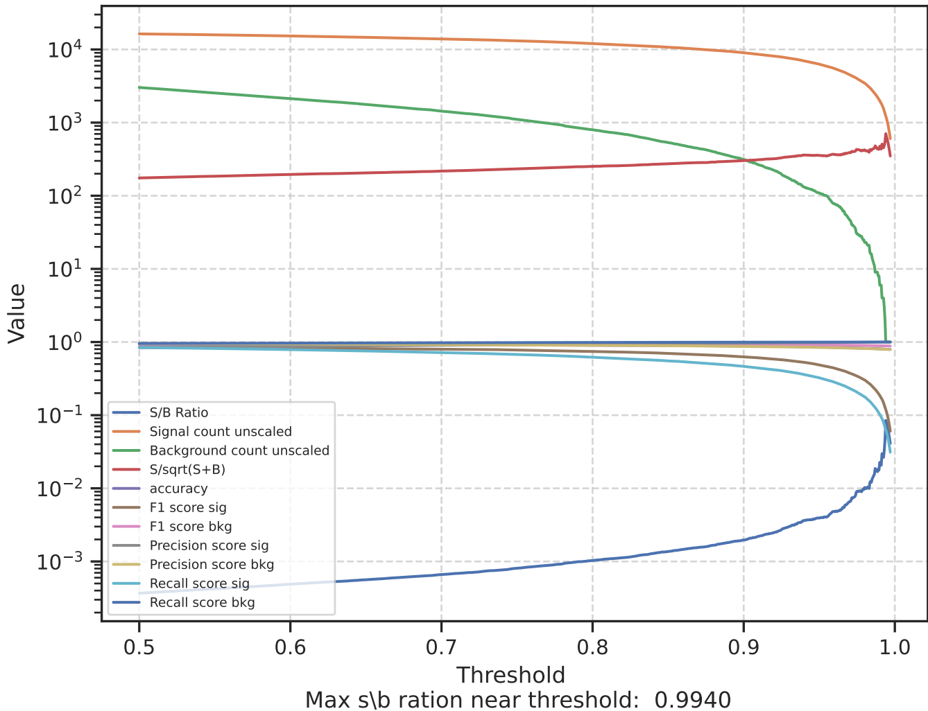
Metrics by classification threshold (Val sample)
