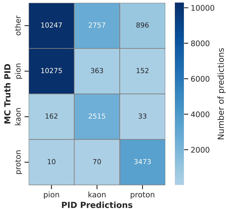
Confusion Matrix
