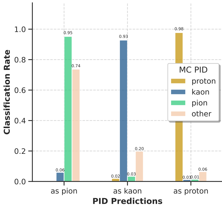
Classification Rate
