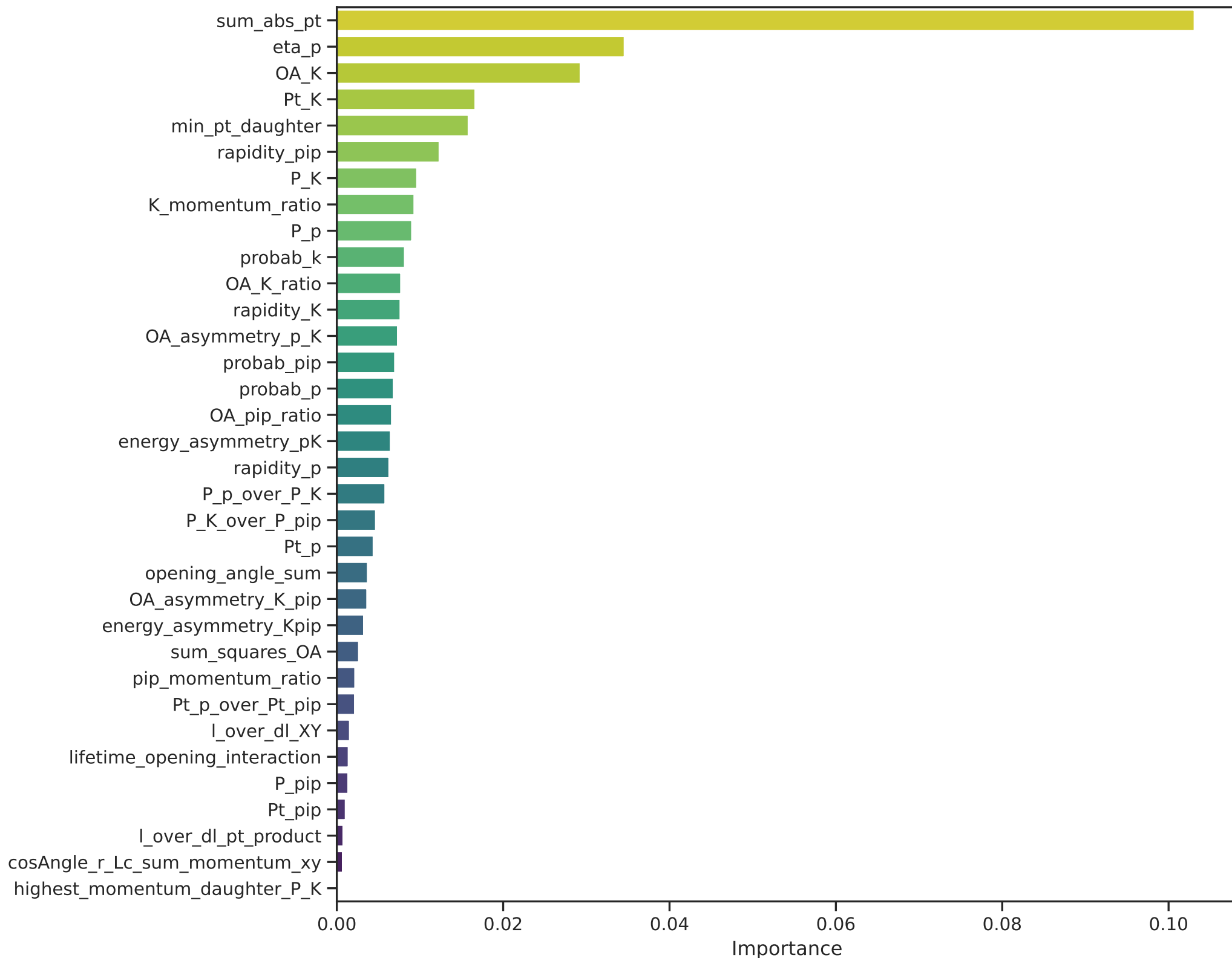
Feature Importances - Permutation Importance (train set)
