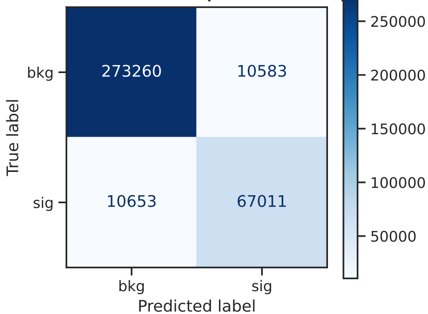
Confusion Matrix (threshold=0.5)
