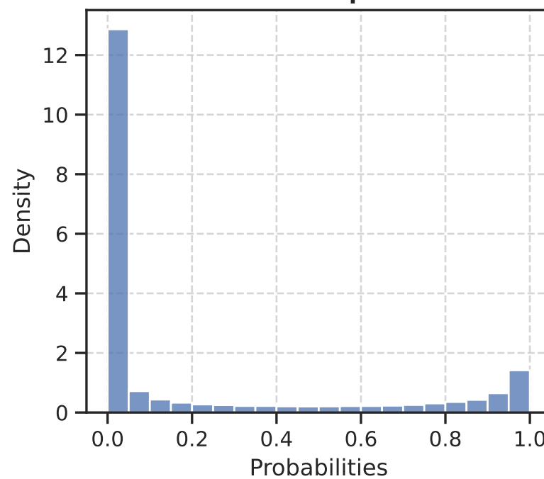
Calbration Plot
