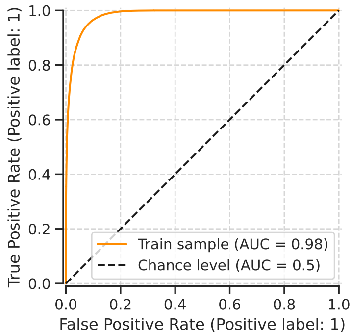
ROC Curve
