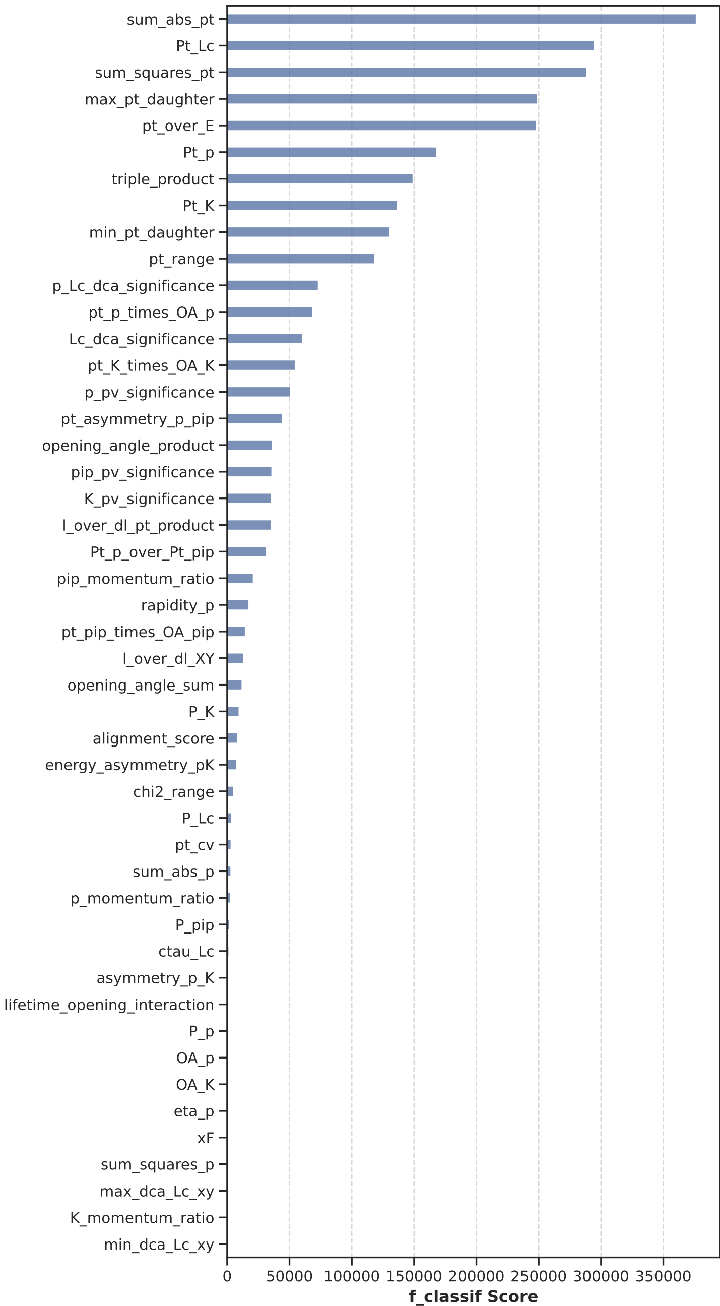
Feature Importance - f_classif Scores
