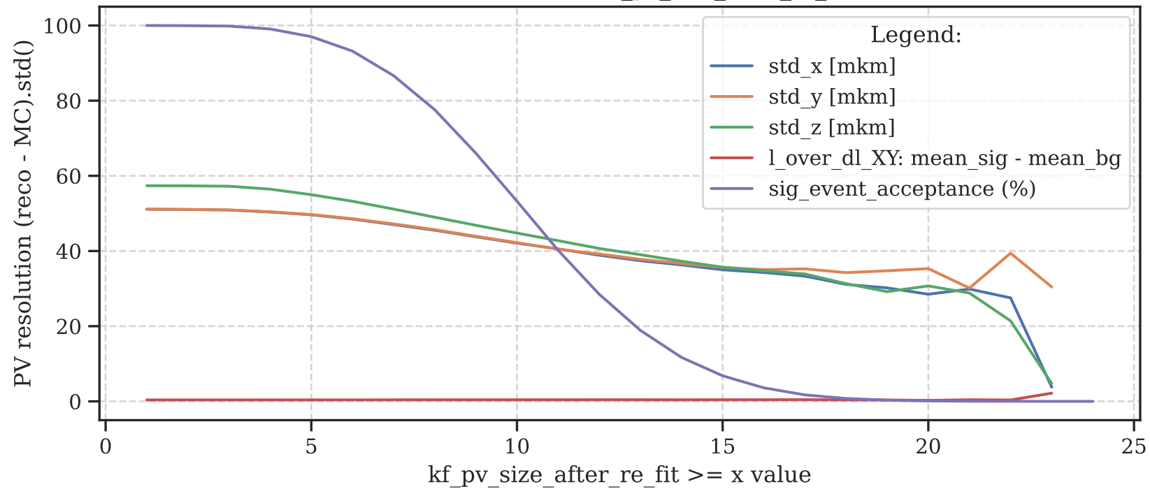
PV Resolution VS. kf_pv_size_after_re_fit
