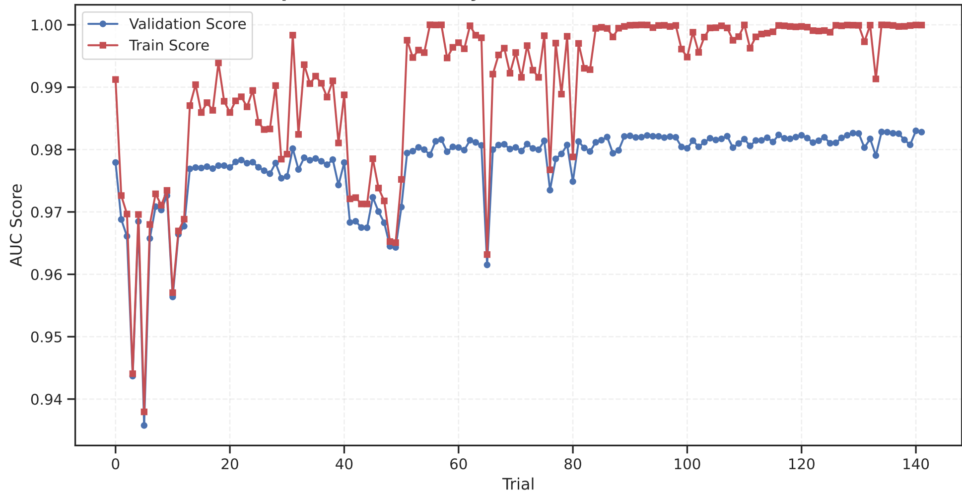
Optimization History - Train vs Validation Scores
