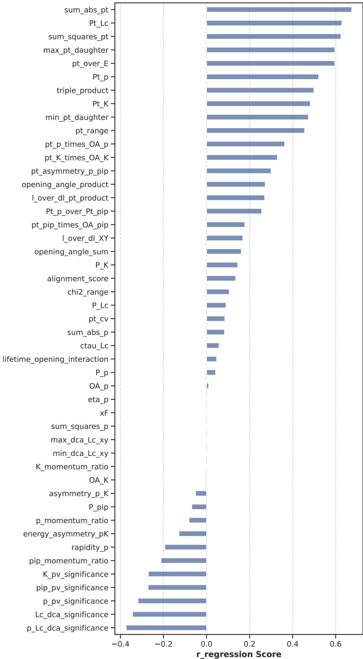
Feature Importance - r_regression Scores
