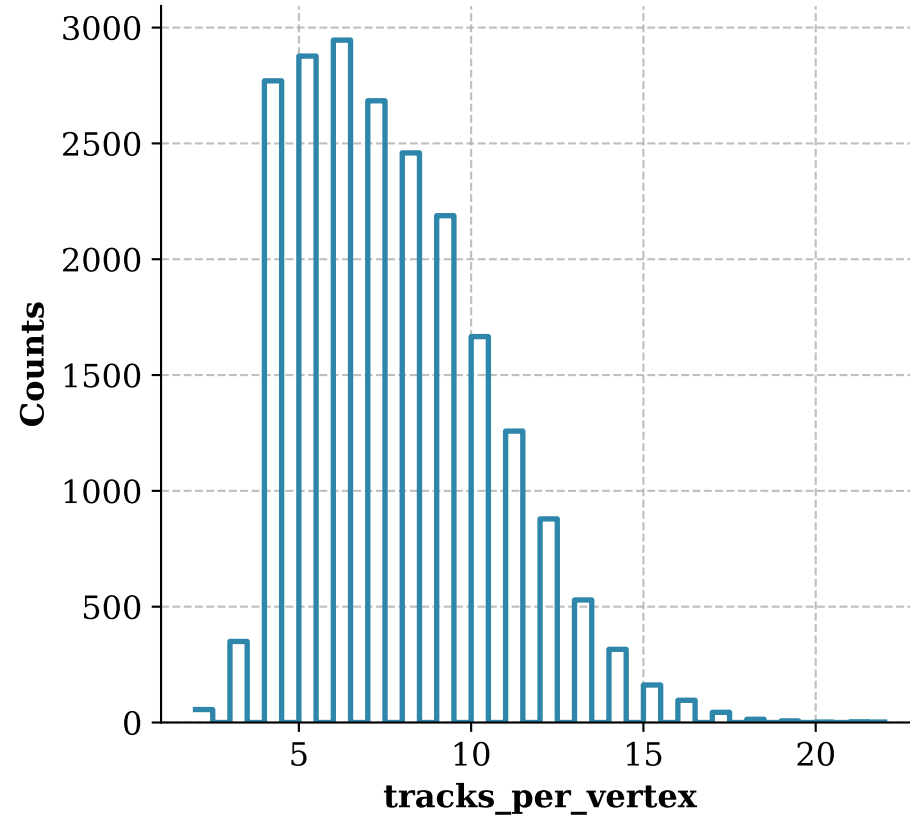
tracks_per_vertex Distribution
