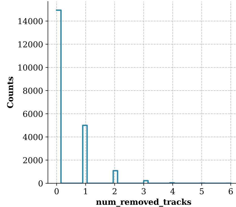
num_removed_tracks Distribution
