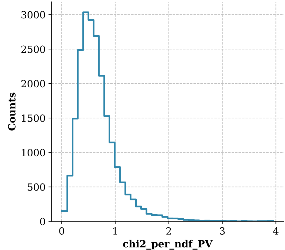
chi2_per_ndf_PV Distribution
