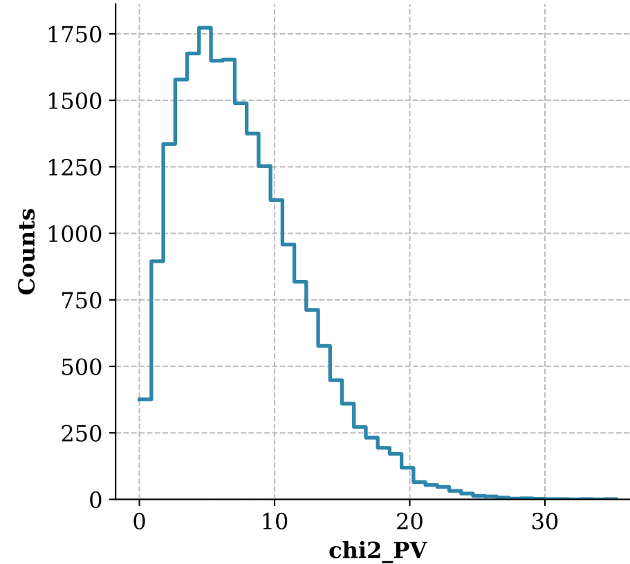
chi2_PV Distribution
