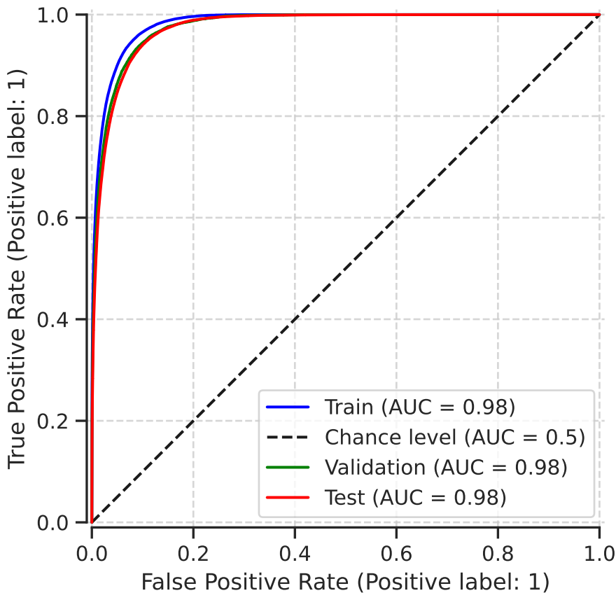
ROC Curve - All Sets
